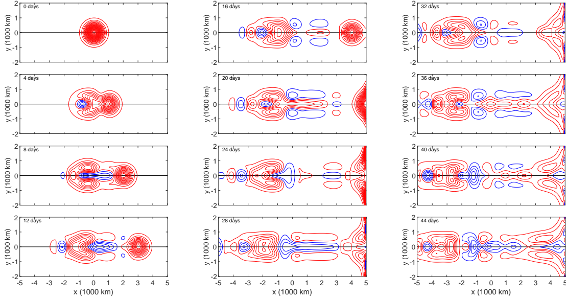
Figure B.2: Evolution of h(x, y, t) starting from a Gaussian perturbation with a_x = a_y = 1 . A time step of 0.02 days was used; positive thermocline thickness anomalies (warm anomaly) are plotted in red contours. Various types of equatorial waves travel along the equator with characteristic phase speeds, and Kelvin waves escape polewards along the eastern boundary of the domain. Once they reach the northern and southern boundaries (not shown), they travel westwards, unless suppressed during the time stepping.
