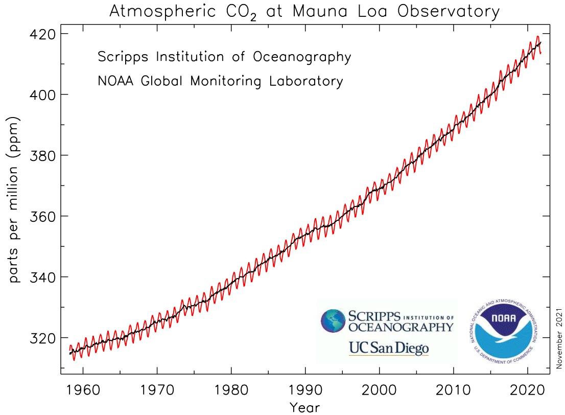
Figure 1.18: Increase in CO 2 concentration, measured since 1958 on Mauna Loa (Hawai'i). CO 2 -data from https://gml.noaa.gov/ccgg/trends/ .
