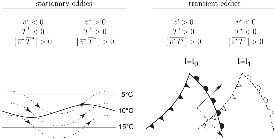
Figure 4.3: Schematic illustration of stationary and transient eddies in the atmosphere. In the situation above, both systems transport heat northwards.
