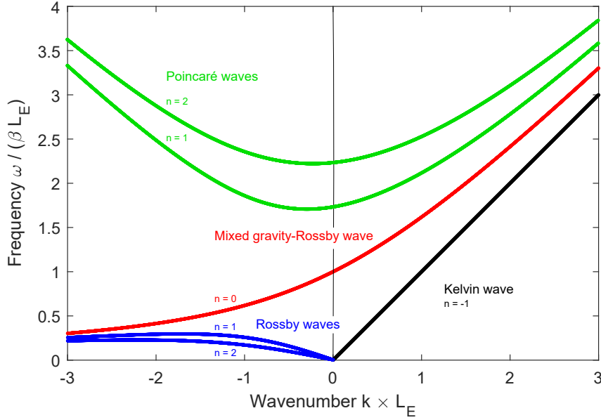
Figure B.1: Dispersion relation of equatorial waves (see end of this problem how to derive it). There are four types of equatorial waves: n \geq 1 modes of each high-frequency gravity waves (Poincaré waves) and low-frequency Rossby waves, and one mode ( n = 0 ) of a mixed gravity-Rossby wave (Yanai wave) and a Kelvin wave ( n = -1 ). Note that for the Kelvin wave the phase speed c_{ph} = \omega/k is only positive, i.e. the phase propagates eastwards), whereas it is strictly negative for the Rossby waves whose phase propagates westward. However, wave energy is transported at the group velocity c_{gr} = \partial\omega/\partial k . Therefore, Rossby and Poincaré waves transport energy in both zonal directions.
