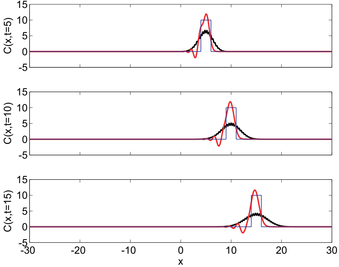
Figure 3.13: Comparison of the exact solution ( thin blue curve ) with different numerical solutions of the advection equation: Lax scheme (3.49) ( black curve ) and Lax-Wendroff scheme (3.53) ( red curve ). The parameters are: \Delta x = 0.2 , \Delta t = 0.1 and u = 1 . The initial condition is C = 1 for -1 \leq x \leq 1 , C = 0 else. The Lax scheme (3.49) exhibits a strong damping and therefore a substantial underestimation of the gradients. The Lax-Wendroff scheme (3.53) overestimates the maximum and shows trailing oscillations. However, the representation of the gradients is significantly improved over the Lax scheme.
