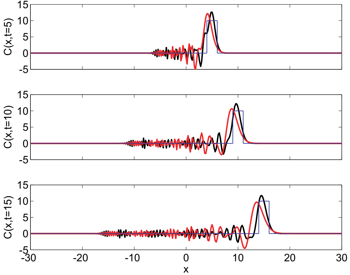
Figure 3.12: Comparison of the exact solution ( thin blue curve ) with the numerical solutions of the advection equation using the implicit-trapezoidal scheme (3.44) with two different time steps: \Delta t = 0.1 ( black curve ) and \Delta t = 0.5 ( red curve ) with \Delta x = 0.2 and u = 1 . The latter violates the CFL criterion, but this is not relevant for the implicit scheme. The initial condition is C = 1 for -1 \leq x \leq 1 , and C = 0 else. Both schemes reproduce the main maximum relatively well, but they also generate numerical modes propagating to the left. The method with the large time step exhibits a greater lag of the main maximum.
