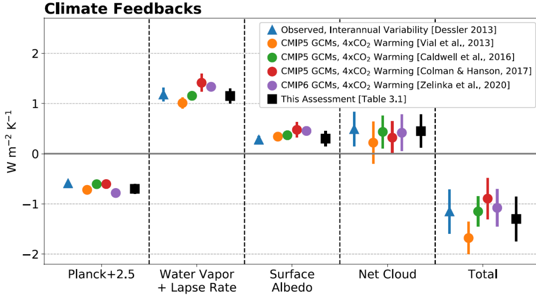
Figure 2.17: Overview of the most important global-scale feedbacks in the atmosphere from observations and various model simulations. Note that the Planck feedback parameter is shifted by 2.5 \text{ W m}^{-2} \text{ K}^{-1} . Results from the present model generation (CMIP6) can be compared to the previous generation (CMIP5). The feedback of the three processes (water vapour+lapse rate, surface albedo, clouds) is overall positive. The total feedback remains, owing to the strongly negative Planck feedback, negative, indicating an overall stable climate system. Figure from Sherwood et al. (2020).
