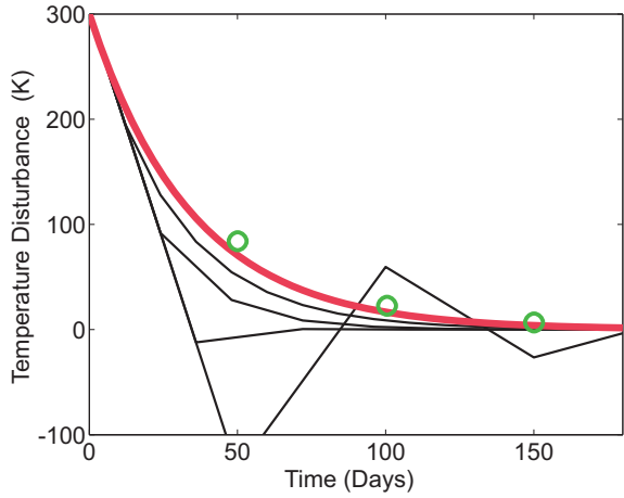
Figure 2.11: Numerical solutions of equation (2.6) with the initial condition \tilde{T}(0) = 300 K computed with the Euler scheme and time steps of 12, 24, 36, 50 days. The exact solution of the linearized system is drawn in a red line , the results from the classical Runge-Kutta scheme ( \Delta t = 50 days) are labelled with green circles .
