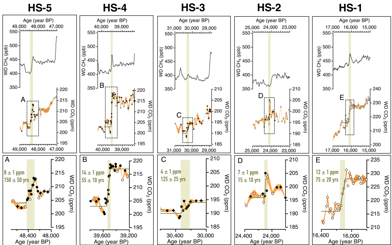
Fig. 2. Centennial-scale \text{CO}_2 and \text{CH}_4 variability during Heinrich Stadials 1 to 5. Upper panel: WD \text{CH}_4 (15), WD \text{CO}_2 from this study (closed circles), and previous publications (open circles) (18, 21) and replicated from previous publications (closed black diamonds). Light orange shading represents pooled 1\sigma standard uncertainty of individual \text{CO}_2 measurements. Shaded vertical bars highlight centennial-scale jumps in WD \text{CO}_2 and \text{CH}_4 . Green lines indicate breakout determinations (see text). Lower panel: WD \text{CO}_2 as in Upper panel sections A–E, with the magnitude and duration of abrupt \text{CO}_2 transitions shown in green.
