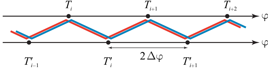
Figure 6.7b: C-grid for the one-dimensional energy balance model.
