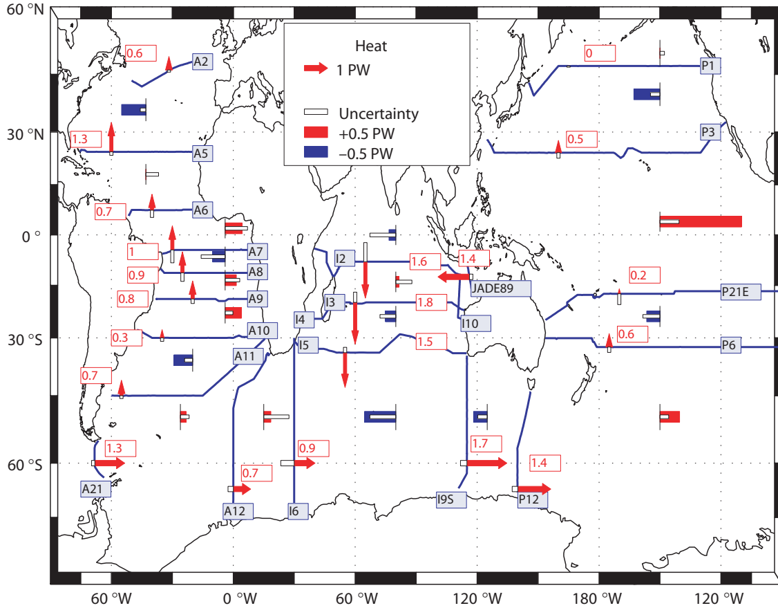
Figure 4.6: Meridional and vertical heat transports in the different regions of the world ocean. Numbers in boxes denote the meridional transport in PW. Horizontal bars represent the vertical transport (to the left = downwards). Figure from Ganachaud and Wunsch (2000).
