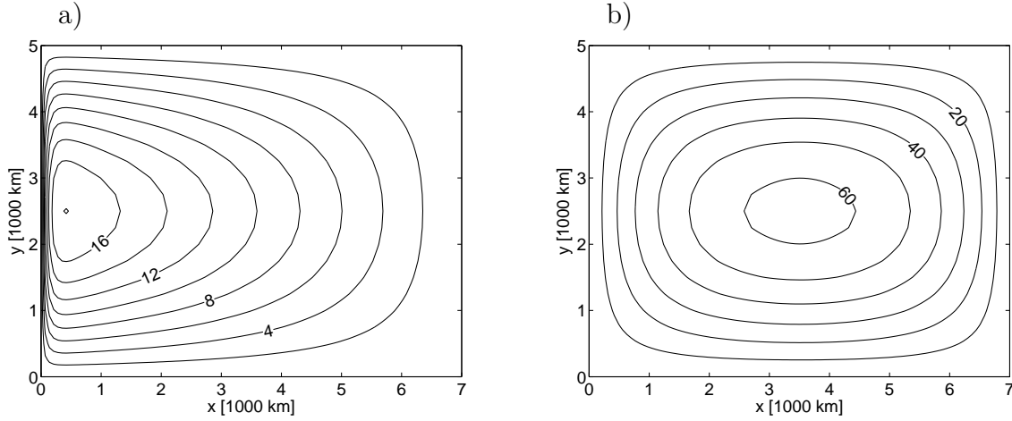
Figure 6.10: Stream function \Psi (in Sverdrup, 1 \text{ Sv} = 10^6 \text{ m}^3 \text{ s}^{-1} ) of the Stommel model (6.40) for a) \beta = 2 \cdot 10^{-11} \text{ m}^{-1} \text{ s}^{-1} and b) \beta = 0 , with R = 1/(6 \text{ days}) , and T = 0.1 \text{ N m}^{-2} in (6.42). The numerical solution was computed on a grid with (N_x = 100) \times (N_y = 20) and using the method of successive overrelaxation (5.22). The current flows clockwise and is parallel to the stream lines.
