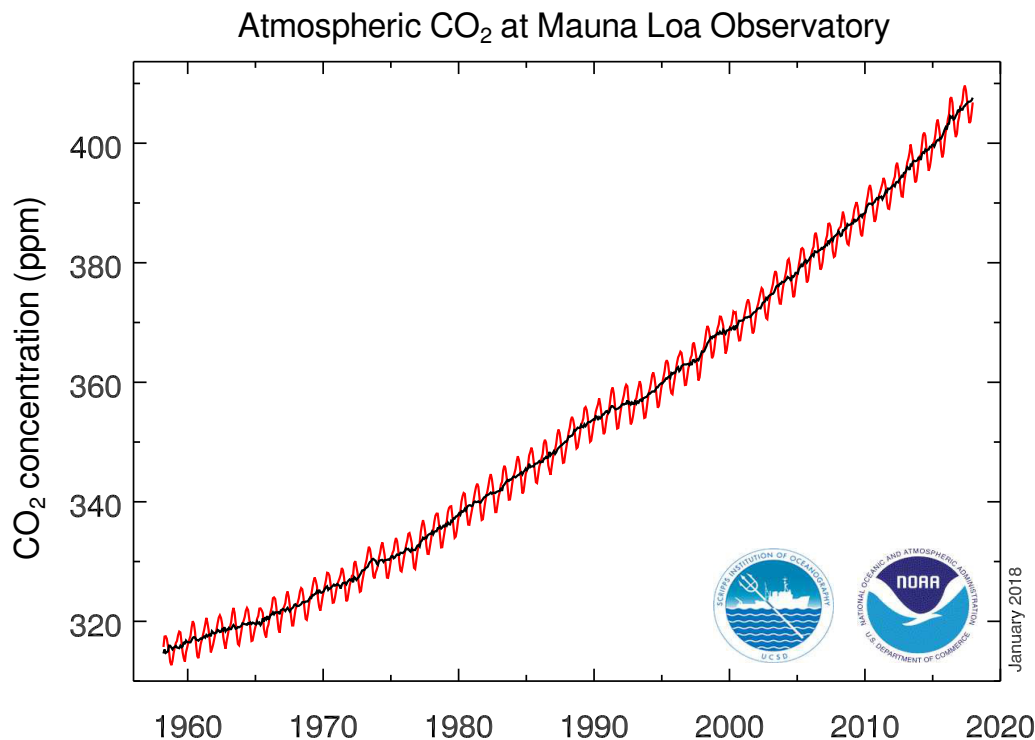
Figure 1.17: Increase in CO 2 concentration, measured since 1958 on Mauna Loa (Hawai'i). CO 2 -data from http://www.esrl.noaa.gov/gmd/ccgg/trends/ .
