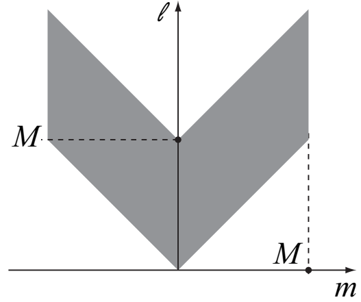
Figure 6.8b: Rhomboidal truncation
