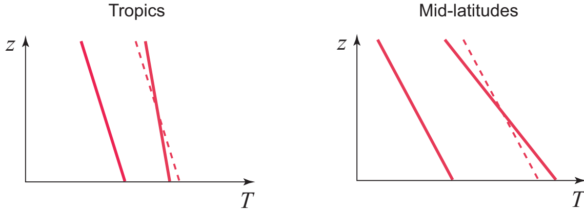
Figure 2.15: Schematic illustration of changes in the vertical temperature structure in the tropics and in the mid-latitudes. Due to increased convection, the lapse rate decreases in the tropics. In the mid-latitudes the horizontal flow limits the warming to the surface and the lower atmosphere which causes the lapse rate to increase. Compared to the mean warming, a reduced warming of the surface occurs in the tropics (therefore a negative feedback), while it is enhanced in the mid-latitudes (positive feedback).
