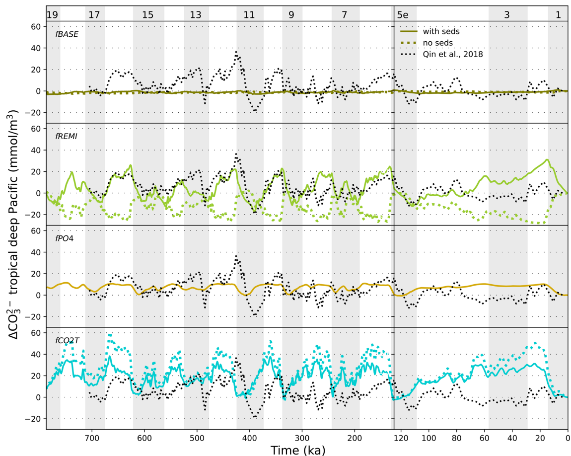
Figure 4. Evolution of \text{CO}_3^{2-} in the tropical deep Pacific as simulated for fBASE, fREMI, fPO4, and fCO2T (from top to bottom) and reconstructed by Qin et al. (2018). The results of the other forcings are shown in Fig. S13.
