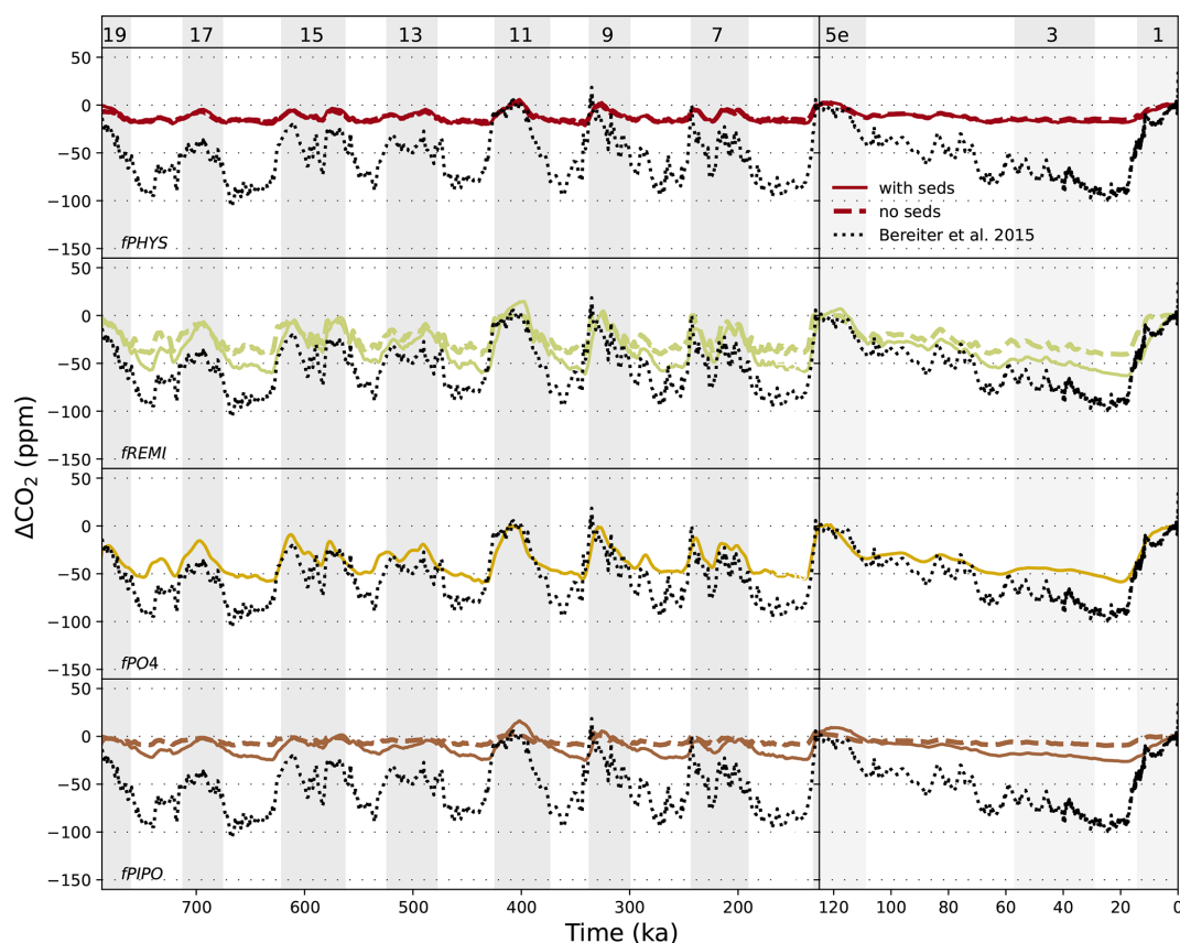
Figure 5. Transient variations in atmospheric CO 2 due to effects fPHYS, fPO4, fREMI, and fPIPO and reconstructed by Bereiter et al. (2015). Shown is the deviation from the pre-industrial value. Grey shading indicates uneven MIS as indicated at the top of the figure. Dashed lines denote runs without the sediment module (not available for PO4). The same plots for the other simulations are shown in Fig. S17.
