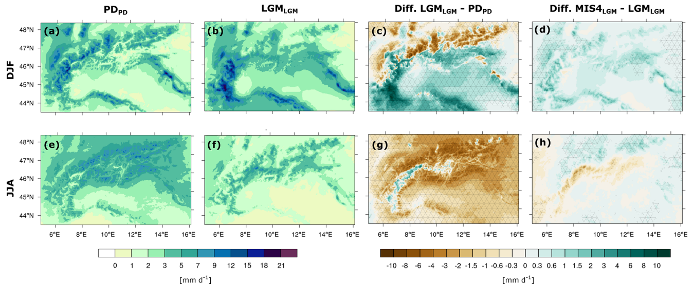
Figure 3. Climatological mean values of daily precipitation intensity over the Alps for (a–d) winter (DJF) and (e–h) summer (JJA): (a, e) the mean PD precipitation, (b, f) the mean LGM precipitation, (c, g) the difference between LGM and PD and (d, h) the difference between MIS4 and LGM. Crosshatched areas represent statistically significant differences with a significance level of 0.05 (using a two-tailed bootstrapping technique).
