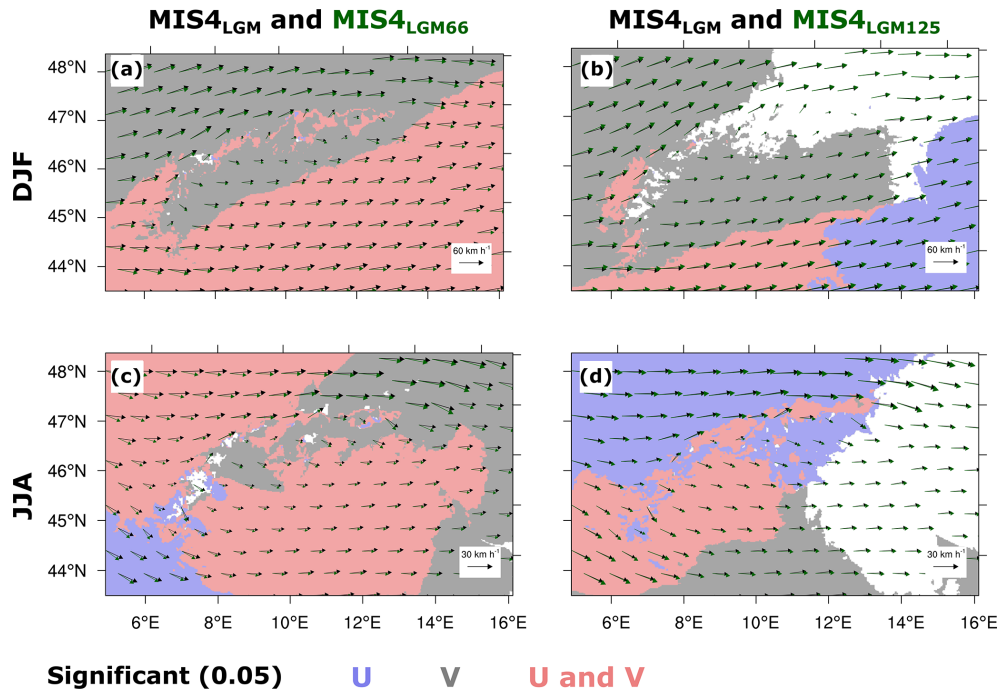
Figure 9. Climatological mean wind vectors over the Alps. Panel (a) represents wind vectors for DJF, black and green vectors correspond to MIS4 LGM and MIS4 LGM66 , respectively, (b) as panel (a) but green vectors to MIS4 LGM125 . (c, d) As panels (a) and (b) but for JJA. Red shading indicates statistically significant differences in zonal ( U ) and meridional ( V ) wind components at a significance level of 0.05 (two-tailed bootstrapping technique), blue and grey shading as the red one but only in U and V wind components, respectively. Please note that the reference wind vectors differ for DJF and JJA.
