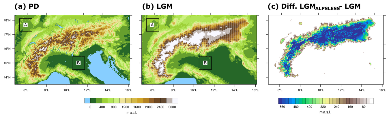
Figure 2. Innermost domain and topography used by WRF. Panel (a) represents the domain at 2 km horizontal resolution and the shading indicates PD topography, (b) as panel (a) but for the LGM topography, crosshatched areas are covered by glaciers. Panel (c) shows the difference between LGM ALPSLESS and LGM topography. The boxes in (a) and (b) are the two regions used for the Skew–T diagrams: Site A represents the north-western and site B the central-southern region.
