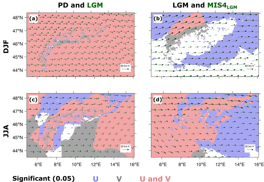
Figure 5. Climatological mean wind vectors over the Alps for (a, b) DJF and (c, d) JJA: (a, c) black and green wind vectors correspond to PD and LGM, respectively, (b, d) black and green wind vectors correspond to LGM and MIS4, respectively. Red shading illustrates statistically significant differences in zonal ( U ) and meridional ( V ) wind components with a significance level of 0.05 (two-tailed bootstrapping technique), blue and grey shadings indicate significance either in the U or V wind component, respectively. Please note that the reference wind vectors differ for DJF and JJA.
