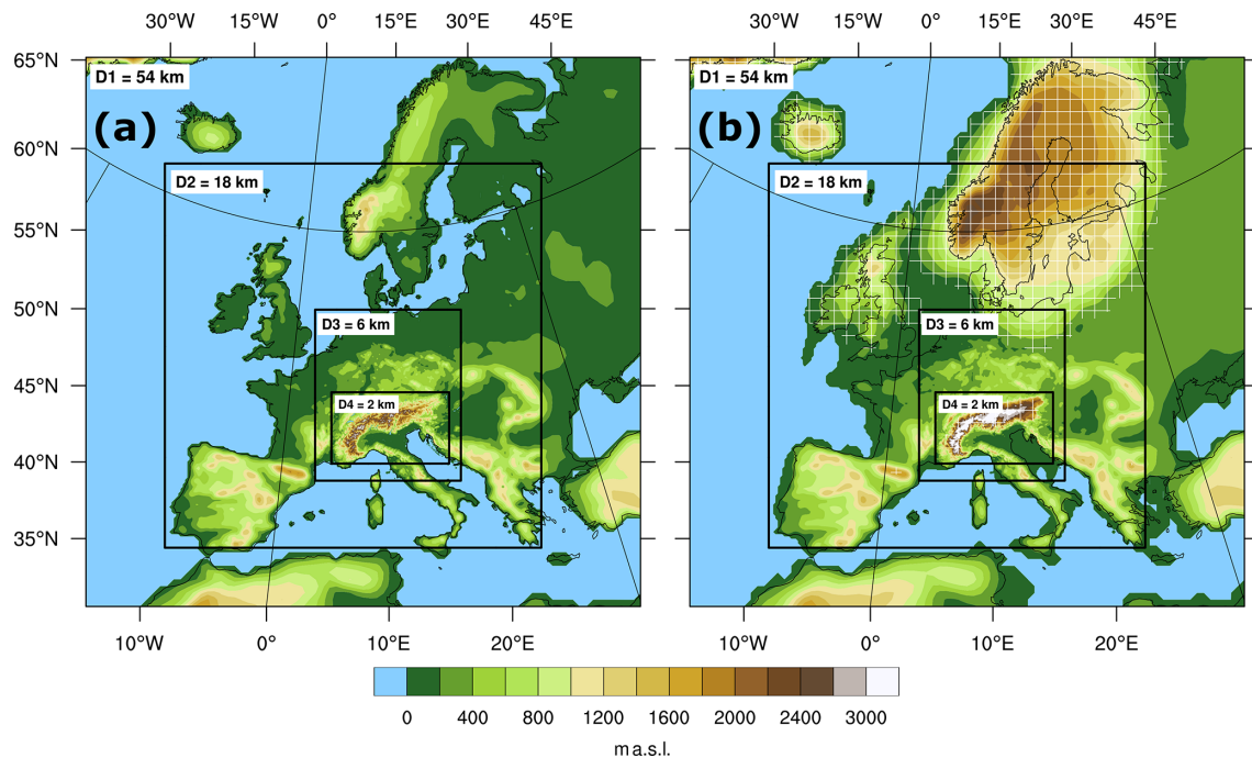
Figure 1. Domains and topography used by WRF. Panel (a) represents the four domains at 54, 18, 6 and 2 km horizontal resolution, and the shading indicates present-day topography; (b) as panel (a) but for the LGM topography, crosshatched areas are covered by glaciers.
