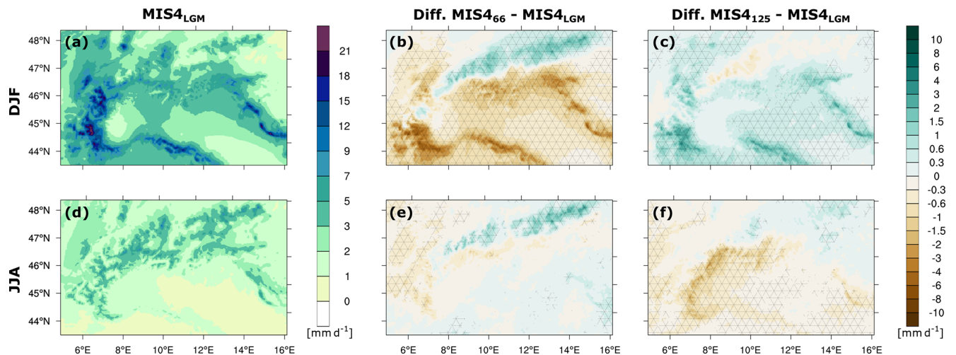
Figure 6. Climatological mean values of daily precipitation intensity over the Alps. Panel (a) represents MIS4_{LGM} precipitation for DJF, (b) the differences between MIS4_{LGM66} and MIS4_{LGM} , (c) as panel (b) but between MIS4_{LGM125} and MIS4_{LGM} . (d, e, f) As panels (a), (b) and (c) but for JJA. Crosshatched areas indicate statistically significant differences at a significance level of 0.05 (using a two-tailed bootstrapping technique).
