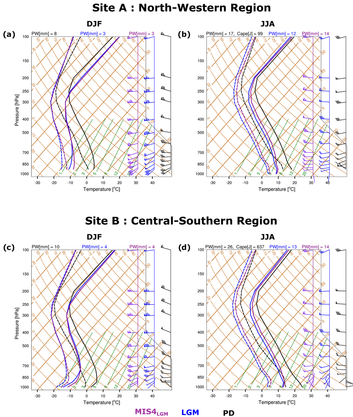
Figure 4. Skew–T diagram for site A (north-western region; a, b ) and site B (central-southern region; c, d ). Sites’ locations are shown in Fig. 2. Panels ( a ) and ( c ) represent climatological vertical profiles for DJF and ( b ) and ( d ) for JJA. MIS4 LGM climate is illustrated by purple lines, LGM climate by blue lines and PD climate by black lines. There are two vertical profiles for each climate: air temperatures in solid lines and dew-point temperatures in dashed lines. Skewed straight dashed green lines represent isohumes labelled on the bottom of the diagram. The mixing ratio is obtained from crossing the saturated mixing ratio lines crossed with the dew-point temperature vertical profile, and its value increases to the right at a constant pressure level. Solid brown lines are isotherms. Dry adiabatic lines (lines of equal potential temperature \theta ) are slightly curved dashed brown lines. In the wind bars, the triangle, line and half-size line represent 50, 10, 5 km h -1 , respectively. Furthermore, vertically integrated precipitable water (PW) and CAPE are given at the top of each panel. Note that CAPE is only displayed if it is different from zero. Please see Sect. 3 for a in-detail description of the Skew–T diagram.
