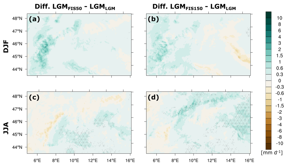
Figure 7. Differences in climatological mean values of daily precipitation intensity over the Alps for (a, b) winter (DJF) and (c, d) summer (JJA): (a, c) LGM_{FIS50} minus LGM_{LGM} and (b, d) LGM_{FIS150} minus LGM_{LGM} . Crosshatched areas indicate statistically significant differences at a significance level of 0.05 (using a two-tailed bootstrapping technique).
