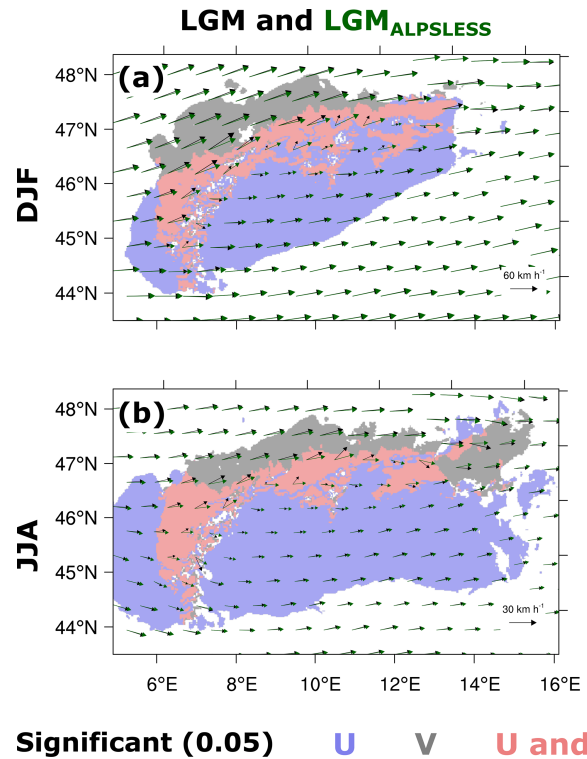
Figure 11. Climatological mean wind vectors over the Alps. Panel (a) represents wind vectors for DJF, black and green vectors correspond to LGM_{LGM} and LGM_{ALPSLESS} , (b) as panel (a) but for JJA. Red shading indicates statistically significant differences in zonal ( U ) and meridional ( V ) wind components at a significance level of 0.05 (two-tailed bootstrapping technique), blue and grey shading as the red one but only in U and V wind components, respectively. Please note that the reference wind vectors differ for DJF and JJA.
