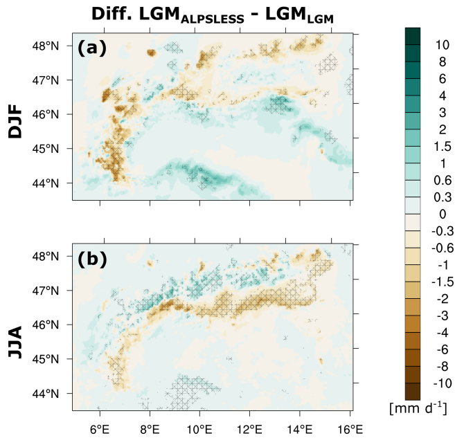
Figure 10. Differences in climatological mean values of daily precipitation intensity over the Alps between LGM_{ALPSLESS} and LGM_{LGM} for (a) winter (DJF) and (b) summer (JJA). Crosshatched areas indicate statistically significant differences at a significance level of 0.05 (using a two-tailed bootstrapping technique).
