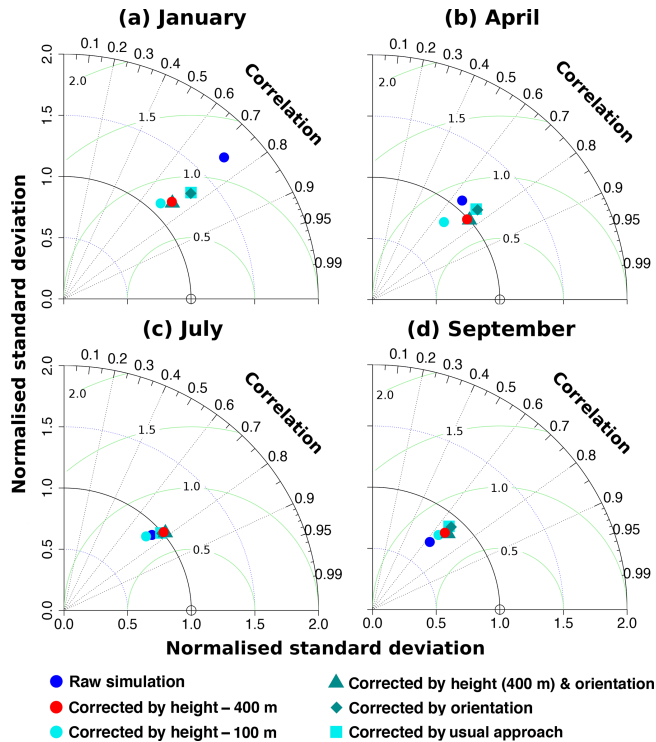
Figure 10. Performance of bias correction with different settings. Panel (a) shows a Taylor diagram for January, (b) for April, (c) for July, and (d) for September. Blue dots represent the raw simulation, red dots the simulation corrected by using height intervals of 400 m, cyan dots the simulation corrected by using height intervals of 100 m, petrol triangles the simulation corrected by using height intervals of 400 m and slope orientations, petrol diamonds the simulation corrected by slope orientations, and cyan squares the simulation corrected by the simple approach (the entire Swiss region). Note that in the Taylor diagram the spatial correlation, spatial root-mean-square error, and spatial standard deviation are shown.
