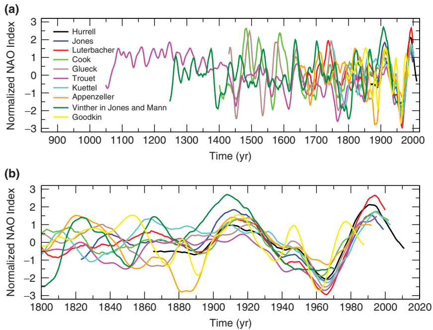
FIGURE 3 | (a) Low-frequency variability of different NAO reconstructions 5,6,16,73–79 for the past millennium and of observations from 1864 to 2009 32 (Figure 2). To focus on low-frequency variations a 31-year time filter is applied to the data except for the NAO reconstructions by Trouet and et al., 6 which only reconstructed the low-frequency variations (also using a slightly different 31-year time filter). Note that the indices of Trouet et al., 6 Hurrell, 32 Cook et al. 74 represent the season DJFM, whereas the others are estimated for the season DJF. Because of the reconstructions methods the variance is underestimated. To make the indices comparable the low-frequency time series are normalized. The Kuettel index 79 is based on selected grid points near Iceland and Lisbon of the sea level pressure fields provided and then the index is calculated similar to the method of Hurrell. 32 (b) As (a) but only showing the period starting 1800.
