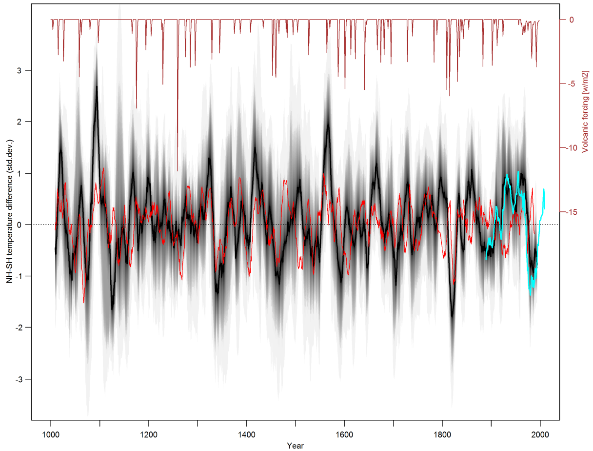
Supplementary Figure 44 | NH-SH differences ECHO-G Erik 2. Same as Supplementary Figure 36 but for the ECHO-G Erik 2 simulation and the corresponding volcanic forcing dataset (Crowley, 2000).
