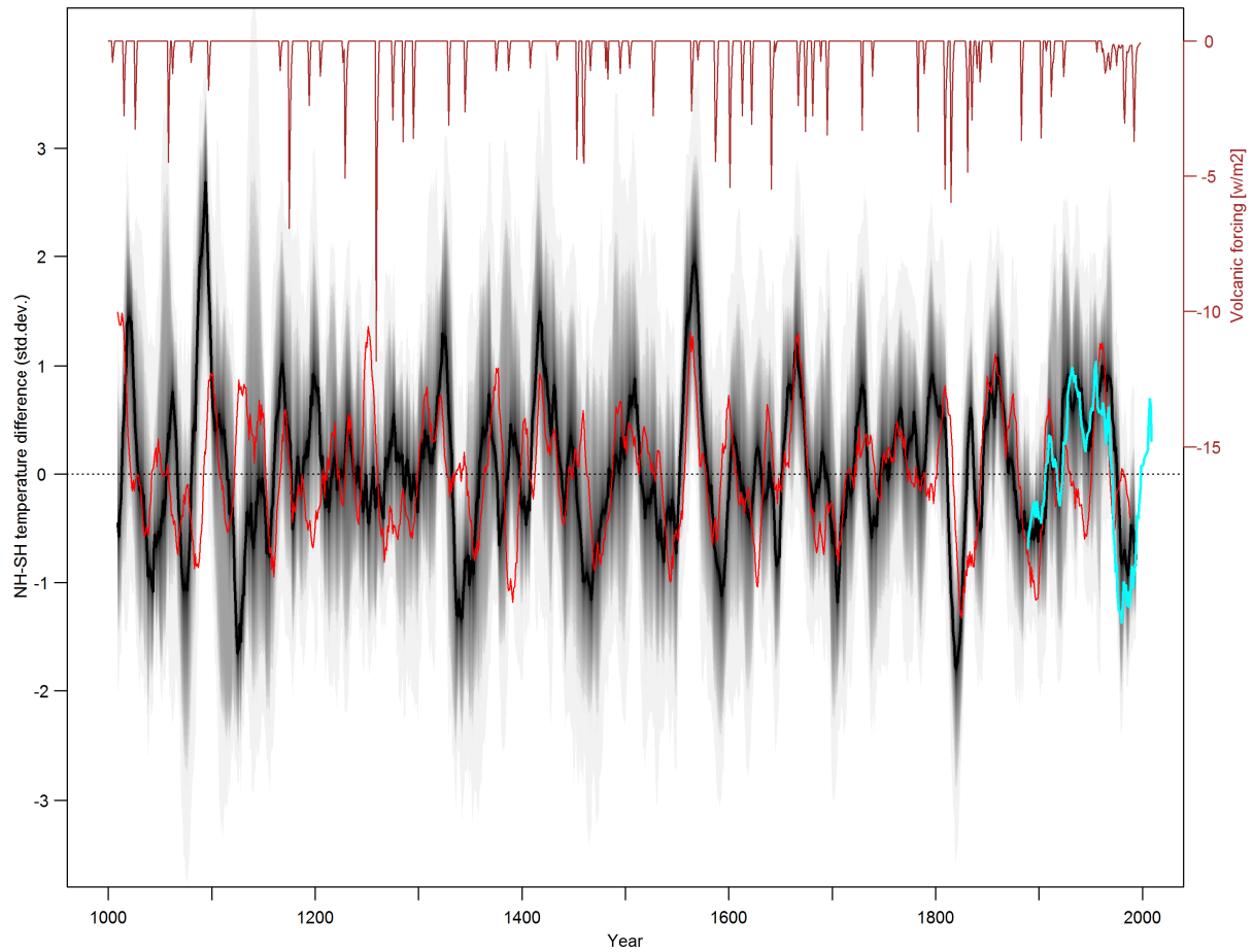
Supplementary Figure 43 | NH-SH differences ECHO-G Erik 1. Same as Supplementary Figure 36 but for the ECHO-G Erik 1 simulation and the corresponding volcanic forcing dataset (Crowley, 2000).
