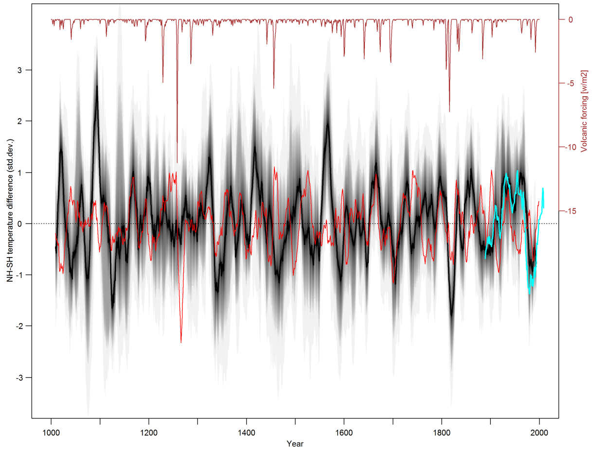
Supplementary Figure 46 | NH-SH differences GISS-E2-R p121. Same as Supplementary Figure 36 but for the GISS-E2-R p121 simulation and the corresponding volcanic forcing dataset (Crowley and Unterman, 2013).
