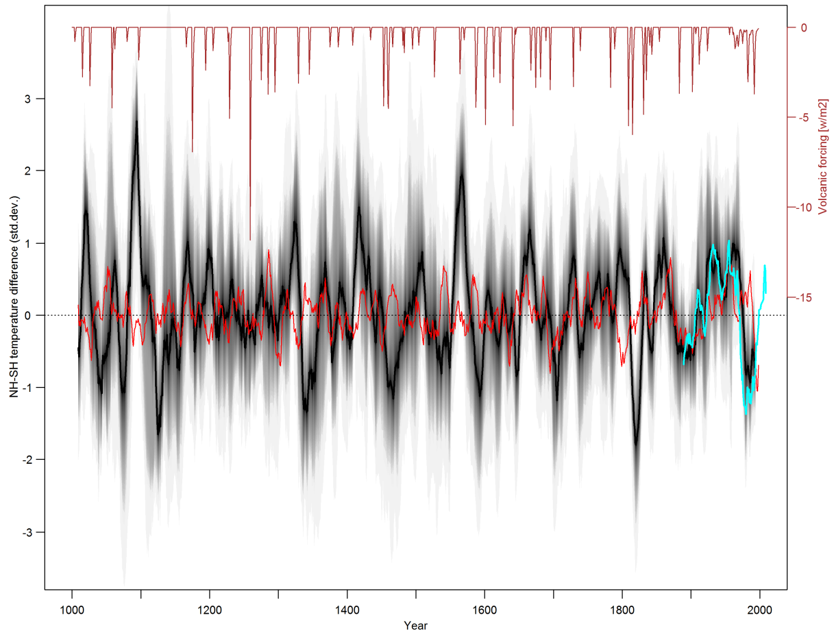
Supplementary Figure 45 | NH-SH differences FGOALS-gl. Same as Supplementary Figure 36 but for the FGOALS-gl simulation and the corresponding volcanic forcing dataset (Crowley, 2000).
