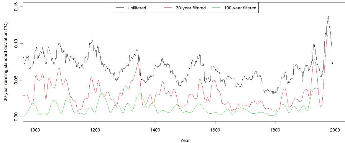
Supplementary Figure 9 | Running standard deviations. 30-year running standard deviations of the unfiltered SH reconstruction ensemble mean (black) and of the 30-year (red) and 100-year (green) loess filtered ensemble mean.
