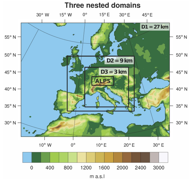
Figure 1. The three nested domains (D1 to D3) with their actual resolution are depicted as black boxes. The box labelled “Alps” denotes the area used for measuring the precipitation intensity of the Vb events. The shading shows the topographical elevation implemented in the simulations in metres above sea level.
