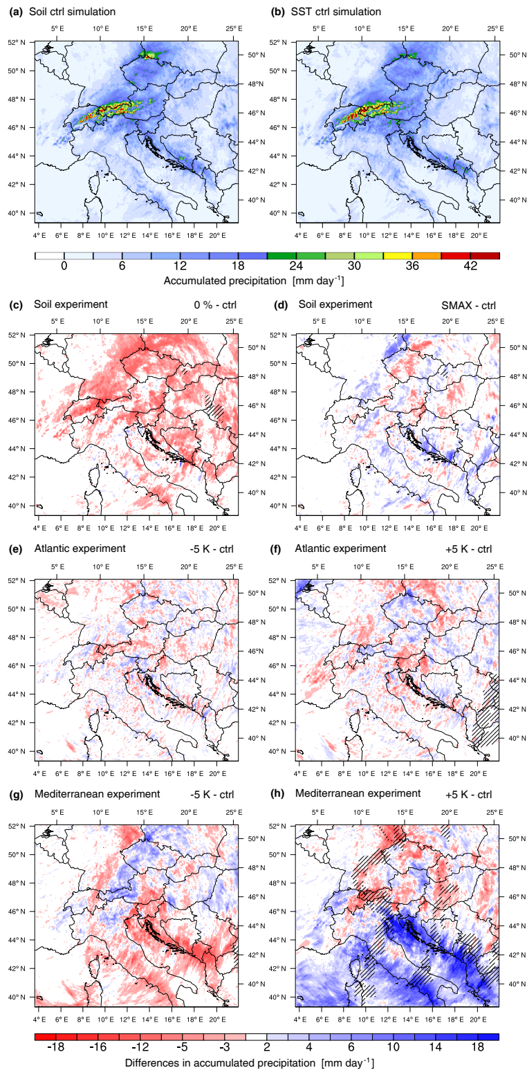
Figure 5. Panel (a) shows the accumulated precipitation ( \text{mm day}^{-1} ) for the control simulation of the soil moisture experiments averaged over the five Vb events. Panel (b) shows the same as panel (a) but for the SST experiments. The second to fourth rows show the differences between the mean daily precipitation obtained by the different sensitivity experiments and the control simulation ( \text{mm day}^{-1} ). Panel (c) shows the complete drainage soil experiment, panel (d) the full saturation soil experiment, panels (e) and (f) the -5 and +5 K Atlantic SST experiments, respectively, and panels (g) and (h) the -5 and +5 K Mediterranean SST experiments. The hatched area denotes significant changes at the 5% significance level using a non-parametric Mann–Whitney U test.
