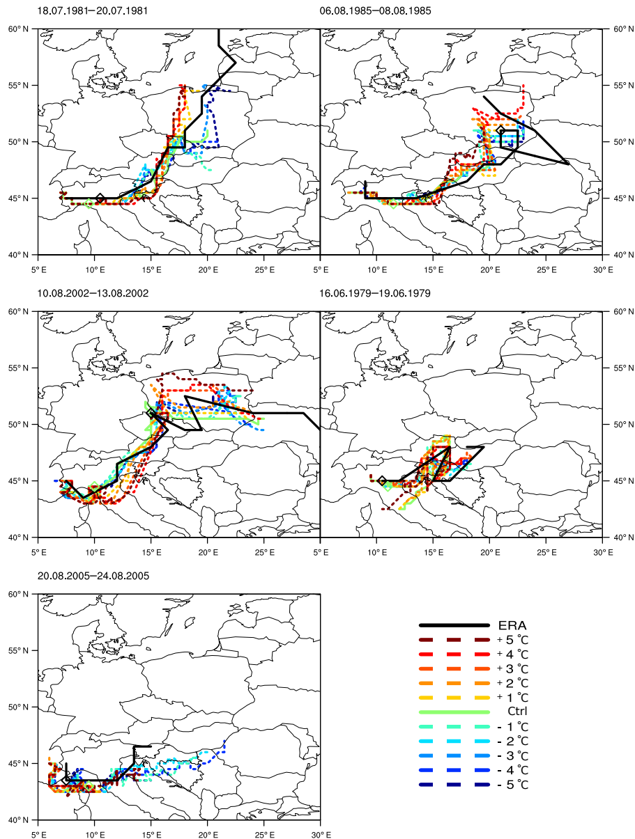
Figure 3. Tracks for the five different Vb events. The black line depicts the tracks that are obtained using the ERA-Interim data set. The light green line shows the tracks detected in the control simulation. The stippled lines show the tracks of the different Mediterranean SST experiments. The green and black diamonds represent the point of the cyclone at which it reaches the strongest gradient during its lifetime for the control simulation and ERA-Interim, respectively.
