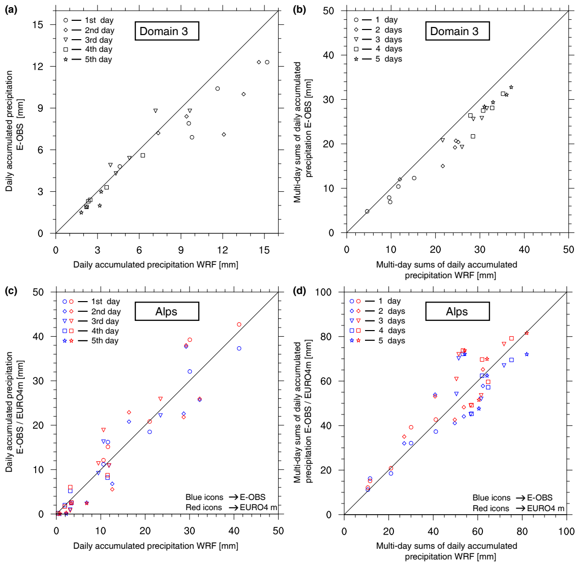
Figure 2. The left column shows the daily accumulated precipitation (mm) obtained by observations plotted against the precipitation obtained by WRF for (a) domain 3 and (c) the Alps (“Alps” box in Fig. 1) for each of the 5 days of the five different Vb events. The right column depicts the multi-day sums of daily accumulated precipitation (mm) for 1 to 5 days for the observations against the multi-day sums obtained by the WRF simulations for (b) domain 3 and (d) the Alps for each of the five Vb events. The upper row uses E-OBS as an observational data set, while the bottom row depicts E-OBS (blue icons) and EURO4m-APGD (red icons) as observational data sets.
