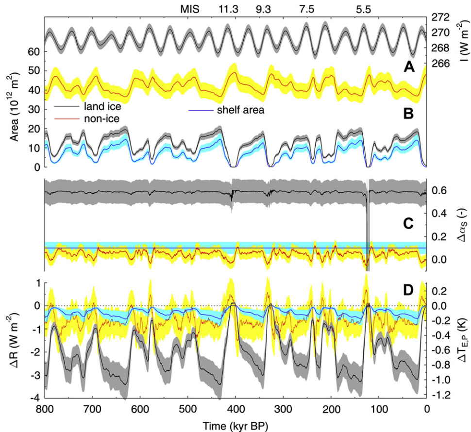
Fig. 3. Albedo feedback from the land cryosphere. (A) Annual mean local insolation at the top of the atmosphere I at 40\text{--}80^\circ\text{N} (Berger, 1978). (B) Area changes of (i) land ice sheets (North America and Eurasia only) and (ii) land without ice (both in 40\text{--}80^\circ\text{N} deconvoluted from the benthic \delta^{18}\text{O} stack LR04 (Bintanja et al., 2005; Lisiecki and Raymo, 2005)), and (iii) global shelf area effected by sea level change based on own assumptions. (C) Changes in surface albedo \alpha_s on areas plotted in (B), those over land ice and ice-free land are again simulation results from Bintanja et al. (2005), while albedo changes on exposed shelves are our own assumption. (D) Perturbation in the radiative budget caused by the albedo feedback from land ice sheets, snow cover on non-glaciated land ( 40\text{--}80^\circ\text{N} ) and sea level change. The right y-axis shows the temperature anomalies \Delta T_{EP} of the Planck feedback. The legend is valid for sub-figures B, C, and D. The albedo over northern hemispheric land ice sheets is undefined around 130 kyr, because these ice sheets disappeared completely. Ice sheets did not vanish completely in the other interglacials, thus albedo over land ice was defined during all other times.
