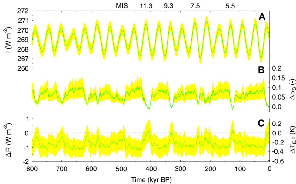
Fig. 5. Vegetation-albedo feedback. (A) Annual mean local insolation at the top of the atmosphere I at 40\text{--}80^\circ\text{N} (Berger, 1978). (B) Changes in surface albedo \alpha_s over vegetation in 40\text{--}80^\circ\text{N} calculated out of continental surface air temperature changes (Bintanja et al., 2005). (C) Perturbation in the radiative budget caused by the vegetation-albedo feedback. Changes are focused on 40\text{--}80^\circ\text{N} . The right y-axis shows the temperature anomalies \Delta T_{EP} of the Planck feedback.
