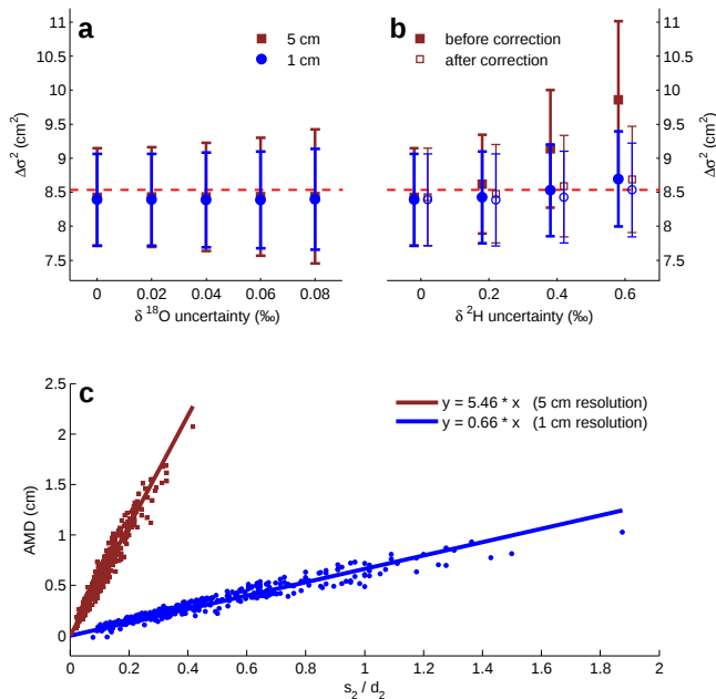
Figure 6. The mean and SD of the differential diffusion length of the 4000 data sets of Monte Carlo run I as a function of the uncertainty in the isotopic measurement are depicted in the top figures. The uncertainty is given as the SD of a Gaussian distribution centred around zero from which random numbers are drawn. The figure on the bottom shows the absolute measurement deviation (as described in the main text) for two different sampling resolutions. The data points given here are obtained from all six Monte Carlo runs and for several assigned values for the uncertainty in the \delta^2\text{H} measurement. The solid lines represent linear regressions to the data points which can be used to correct \Delta\sigma^2 for the deviation that arises as a result of measurement uncertainty.
