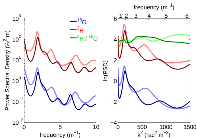
Figure 2. The power spectral densities of two stacked precipitation records retrieved from the GNIP database. In light colours the Debreceen data are given; dark colours refer to data from Vernadsky. The figure on the left shows the PSD as a function of frequency, whereas the figure on the right shows the natural logarithm of the PSD as a function of the wave number squared (bottom x axis).
