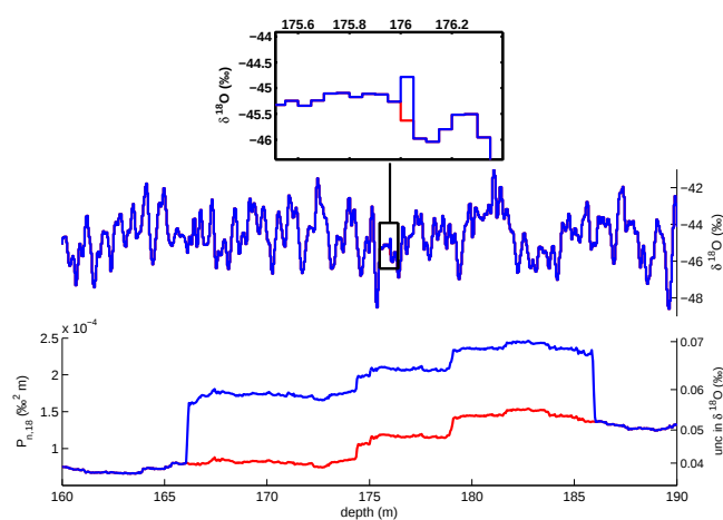
Figure 9. Part of the \delta^{18}\text{O} record (top figure) and the corresponding noise level (bottom figure) that is determined as the average PSD level for frequencies higher than 8 cycles \text{m}^{-1} . The noise level is calculated with a window of 20 m length. The sudden steps in the blue profile are caused by a single data point. Replacing this data point (see inset) by a value obtained by interpolating the neighbouring points leads to a much lower noise level (red curve).
