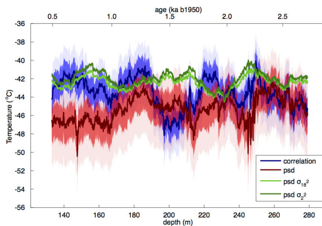
Figure 11. Local surface temperature reconstructions based on the differential diffusion lengths given in Fig. 10 and the model described in the main text. The shaded bands give the 1\sigma and 2\sigma uncertainties and are based on the uncertainty in the differential diffusion lengths. Also given are temperature reconstructions obtained with the PSD method applied to single isotopes (green lines). The recent measured annual temperature at EDML is -44.6^\circ\text{C} . The age scale on the top x axis is the AICC2012 age scale.
