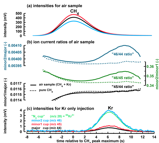
Fig. 4. Comparison of a \text{CH}_4 peak of an air sample with the signals gained from an injection of pure Kr measured with the Bern system at \text{CO}_2 focusing. (a) Beam intensities in mV for the \text{CH}_4 sample peak (369 ppb \text{CH}_4 with natural abundance of Kr) with the retention time centred to the \text{CH}_4 peak maximum. (b) Background-corrected ion current ratios (“46/44 ratio” in blue, “46/45 ratio” in green and “45/44 ratio” in black) of the atmospheric air sample (solid line) and pure \text{CH}_4 (dotted line), illustrating the anomalies seen in “46/44” and “46/45” but with no visible effect on “45/44”. Panel (c) shows the beam intensities for a measurement where Kr was injected into the GC flow. Due to the chromatographic effect of the GC column, the retention time of the Kr peak is ca. 6 s longer than the \text{CH}_4 peak, yet there is a considerable overlap. Note the signal measured at m/z 28 (“ \text{N}_2 cup”) can be directly related to ^{84}\text{Kr}^{3+} , which has the exact value of m/z = 28 .
