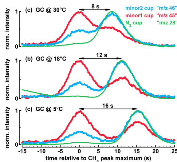
Fig. 8. Chromatograms showing the separation between \text{CH}_4 (left peak) and Kr (right peak) on a PoraPLOT column for 30^\circ\text{C} , 18^\circ\text{C} and 5^\circ\text{C} measured with the Bern system. The Kr interference is visible in all Faraday cups, either as a direct signal of ^{84}\text{Kr}^{3+} in the m/z 28 cup (thin green line) or from the broad Kr interference for the minor1 and minor2 (thick red and blue, respectively).
