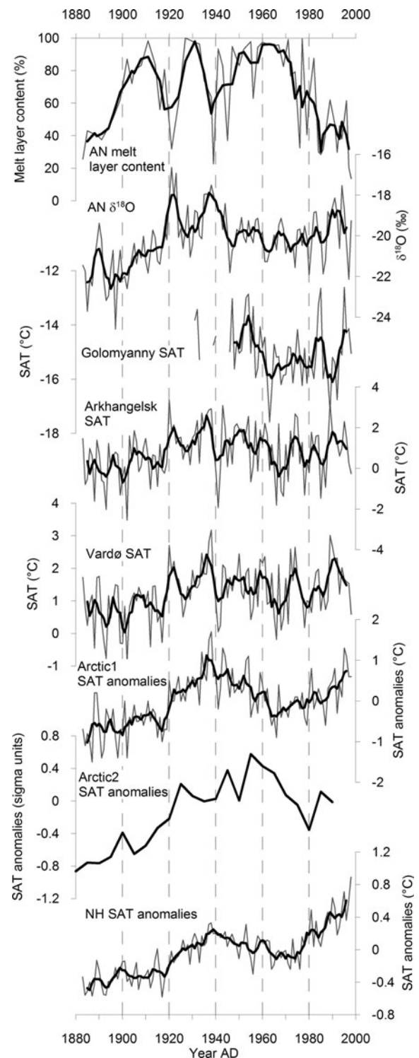
Fig. 5. Time series of the AN melt-layer content, AN \delta^{18}\text{O} , sub-Arctic and Arctic SAT and NH SAT. The thin grey lines indicate annual mean values. The thick black lines represent 5yr values (for AN melt-layer content 1 and 3 m running mean values, respectively) except for Arctic2, where it represents 5 year mean values. Arctic1 displays the Arctic SAT anomalies (relative to 1961–90) dataset of Polyakov and others (2003b), Arctic2 the reconstructed Arctic SAT anomalies (relative to 1901–60) of Overpeck and others (1997).
