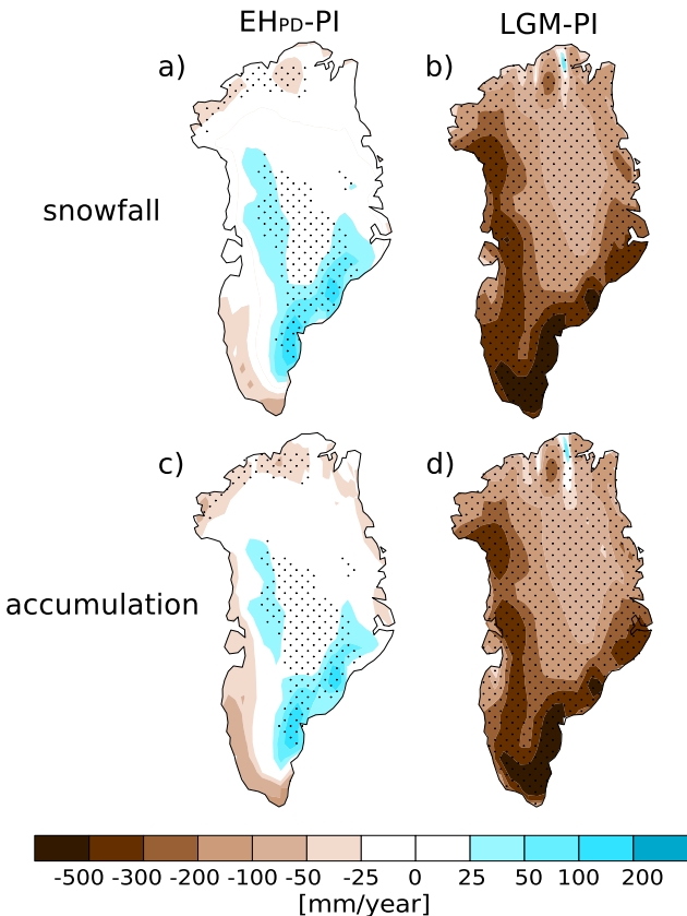
Fig. 4. Annual mean (a, b) snowfall and (c, d) accumulation [mm yr −1 ] anomalies for EH PD -PI and LGM-PI. Stippling denotes values significant at the 5 % level based on t -test statistics.
