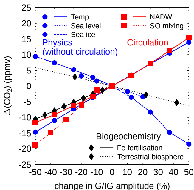
Fig. 10. Sensitivity analysis of the impact of the glacial/interglacial amplitudes of the individual processes on the rise in atmospheric CO 2 during the last glacial/interglacial transition covering Termination I (30–0 kyr). The figure shows the differences in the rise in CO 2 between scenarios (all processes included) with variable amplitude in one process and scenario S1.5K. Processes depict changes in ocean temperature (Temp), sea level, gas-exchange rate through sea ice, NADW formation, Southern Ocean vertical mixing, Fe fertilisation in the Southern Ocean, and carbon storage in terrestrial biosphere. Note, that the carbonate compensation is a response process and cannot be modified in its amplitude. Glacial/interglacial amplitude of sea level change was varied only \pm 20\% due to high reliability of known sea level change. The glacial/interglacial amplitudes of iron (Fe) fertilisation, and Southern Ocean vertical mixing (Southern Ocean mixing) could only be reduced as they were operating on their possible upper limit.
