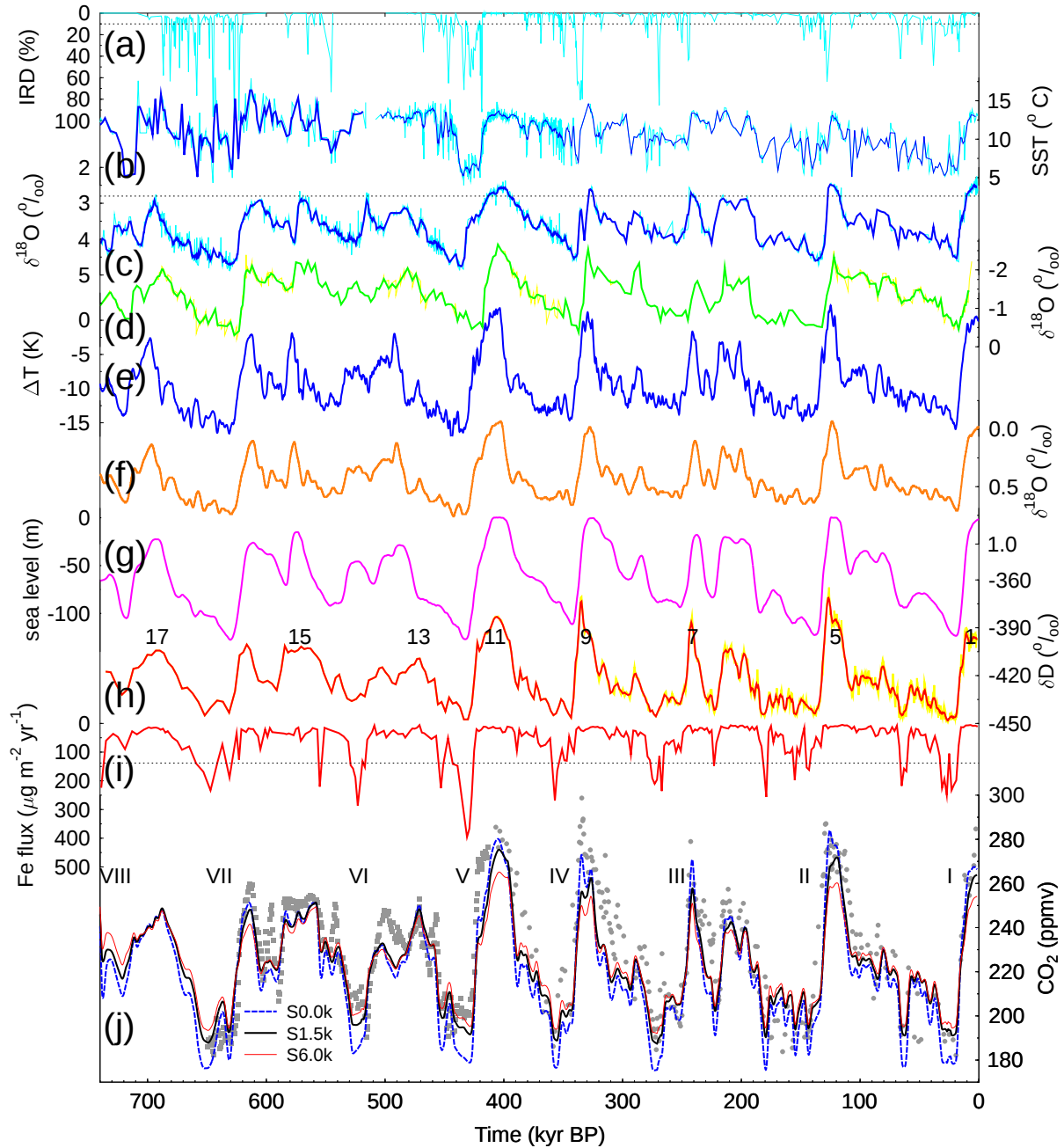
Fig. 2. Paleo-climatic records which were used to force the BICYCLE model ( a–i ) and measured and simulated CO 2 ( j ). Ice rafted debris IRD ( a ), SST reconstructions ( b ), and benthic \delta^{18}\text{O} in foraminifers ( c ) from the sediment core drilled at the site ODP980 (55°29' N, 14°42' W) (McManus et al., 1999; Flower et al., 2000; Wright and Flower, 2002). ( d ): Planktic \delta^{18}\text{O} of ODP677 (1°12' N, 83°44' W) (Shackleton et al., 1990). Reconstructed ( e ) temperature changes over land in the northern hemisphere (40–80° N), ( f ) variability in deep ocean \delta^{18}\text{O} caused by deep ocean temperature changes, and ( g ) sea level changes, ( e–g ) after Bintanja et al. (2005). Sea level corrected deuterium \delta\text{D} ( h ) and atmospheric iron fluxes to Antarctica ( i ) as measured in the EPICA Dome C ice core (EPICA-community-members, 2004; Wolff et al., 2006). ( j ): Measured CO 2 from Vostok (grey circles) (Petit et al., 1999) plotted on the orbitally tuned age scale (Shackleton, 2000), from EPICA Dome C (grey squares) (Siegenthaler et al., 2005), and simulated CO 2 (lines, 3 kyr running mean) of scenarios with different response time of the carbonate compensation: S0.0K: instantaneous response; S1.5K, S6.0K: response delayed by an e-folding time of 1.5 and 6 kyr, respectively. Data prone to high frequency fluctuations ( b , c , d , h ) were used as 3 kyr running means. Fe fluxes used as published as 2 kyr averages. Numbers in panel ( h ) label interglacial MIS, the Latin numbers in panel ( j ) count the last eight terminations. Horizontal lines (in a , c and i ) mark certain thresholds.
