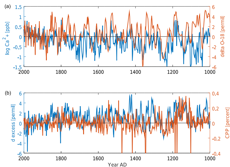
Figure 7. Records of KCC, displaying \delta^{18}\text{O} together with \text{Ca}^{2+} (a) and deuterium excess together with the coarse particle percentage (CPP, b), shown in blue and orange, respectively. All time series are shown as anomalies relative to the respective AD 2000–1860 mean at biennial resolution. Note the high levels of deuterium excess and CPP around AD 1100–1200.
