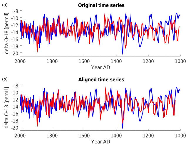
Figure 5. Stable water isotope time series of KCC and KCI, shown in blue and red, respectively: (a) shows both records on their original timescale over the last 1000 years; (b) the KCI age scale was adjusted using the algorithm of Lisiecki and Lisiecki (2002) to optimize the match with KCC.
