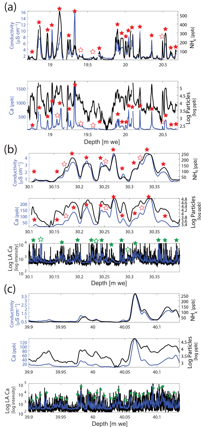
Figure 3. Examples for annual layer counting in KCC impurity profiles for three different depth sections, labelled (a), (b) and (c), and corresponding roughly to 100, 250 and 1000 years before 2013, respectively (see Table 3). In the upper core parts (firm sections) CFA measured impurities were used for counting, with special emphasis on \text{NH}_4^+ (a). Counted years are marked as full stars and uncertain years as white stars. (b) The middle row shows an example of overlap in counting between CFA and LA-ICP-MS Ca, showing (10 \pm 3) and (11 \pm 3) years, respectively. The LA-ICP-MS Ca raw signal is shown in black together with Gaussian smoothing (blue). Note that a minor depth offset (at most a few centimetres) may exist between the CFA and LA-ICP-MS datasets. Accordingly, no one-to-one match of the individual peaks is attempted. Counting within one of the deepest sections analysed for this study is shown in (c). Here, only the LA-ICP-MS Ca allows a reliable identification of almost sub-centimetre thin annual layers. LA-ICP-MS intensity is reported as counts per second.
