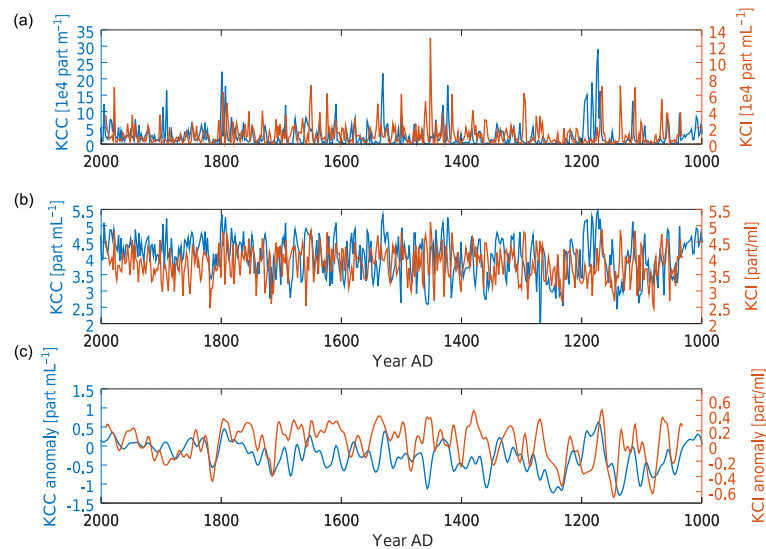
Figure 8. Inter-core comparison of the insoluble particle signal of KCC (blue) and KCI (orange): (a, b) show the insoluble particle time series on a linear and logarithmic scale, respectively; (c) shows decadal trends of anomalies with respect to their AD 2000–1860 mean, highlighted by Gaussian smoothing. The KCI record is on the adjusted timescale after matching the stable water isotope records.
