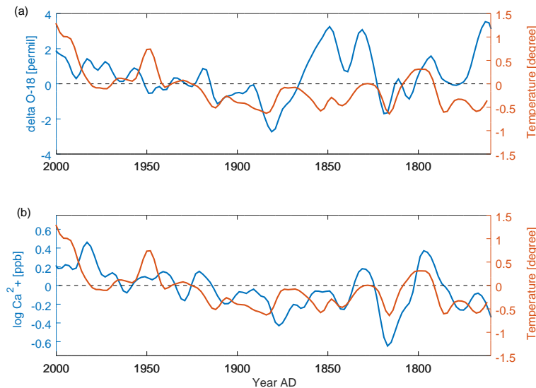
Figure 6. Comparison of KCC \delta^{18}\text{O} and \text{Ca}^{2+} against the CG modified instrumental temperature (orange), shown in (a) and (b), respectively, and covering the full instrumental period back to AD 1760. Anomalies are shown relative to the respective AD 2000–1860 mean, and as decadal trends obtained from Gaussian smoothing.
