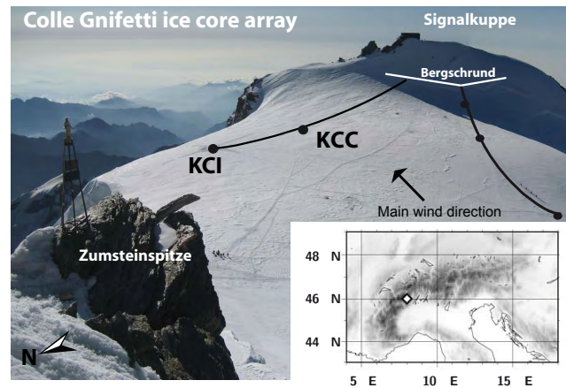
Figure 1. The ice core array at Colle Gnifetti, at 4450 m a.s.l. in the Monte Rosa summit range. The drilling sites of the two cores KCI and KCC are located on approximately the same flow line (black line) towards the eastern flank (downwind of the main wind direction), hence providing the same upstream catchment area. Locations of previous drillings initiated by the Institute of Environmental Physics are also shown as small black dots for reference.
