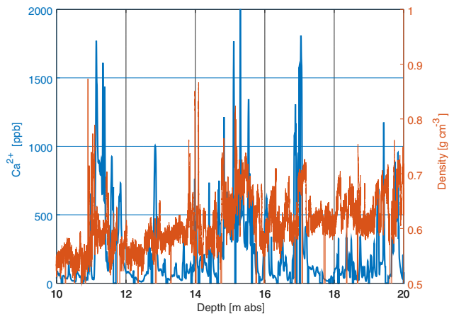
Figure 10. Example view on comparing the KCC \text{Ca}^{2+} record with the density profile. Density was measured at high resolution by computer tomography at the Alfred Wegener Institute Bremerhaven (Johannes Freitag, personal communication, 2017). The comparison illustrates the connection between dust content and presumed faster snow consolidation: layers of high dust load coincide with layers of enhanced density (with respect to ambient layers).
