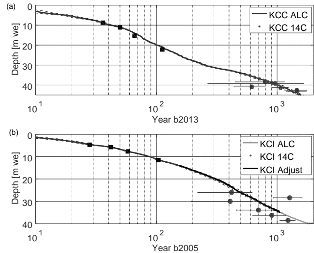
Figure 4. Age–depth relations over the last 1000 years for KCC (top) and KCI (bottom). Age is plotted on a logarithmic axis, together with the according estimates of maximum dating uncertainty (dashed lines) and ^{14}\text{C} age constraints (with 1\sigma range) for KCC and KCI. Also shown is the adjusted age scale of KCI based on the stable water isotope time series comparison (solid black line, within less than 15 years of the original dating and thus hardly distinguishable here; see text). Absolute dating horizons used roughly within the last 100 years (see text) are shown as black squares. Note that the KCI chronology is based on a simple extrapolation below 26 m w.e. and has large uncertainty beyond the last 1000 years (thus indicated as light grey line only).
