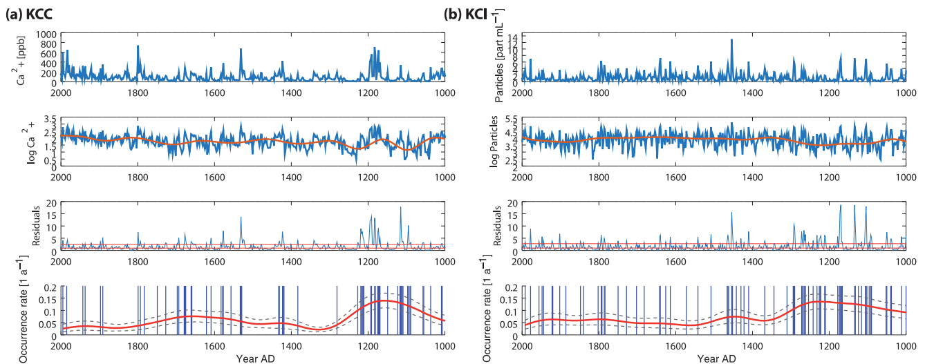
Figure 9. Results from detecting Saharan dust events in the ice core records and estimating their long-term frequency of occurrence: (a) corresponds to KCC and (b) to KCI (see text). The bottom row shows the detected events (blue) and the frequency of occurrence kernel estimate with a 51-year bandwidth (bottom rows, in red) together with 90% confidence intervals.
