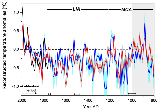
Figure 11. Comparison of decadal temperature trends as anomalies with respect to the mean of AD 2006–1860. Shown are calibrated temperatures obtained from the KCC \text{Ca}^{2+} variability (blue lines, with uncertainty indicated as light blue bands). Also shown are instrumental temperature data (black) and the summer temperature reconstruction of Luterbacher et al. (2016) in red (uncertainty as grey bands). Note that the overall co-variation between the two reconstructions persists for at least another 200 years beyond AD 1000 (light grey shaded area). Black bars on the bottom indicate maximum dating uncertainty.
