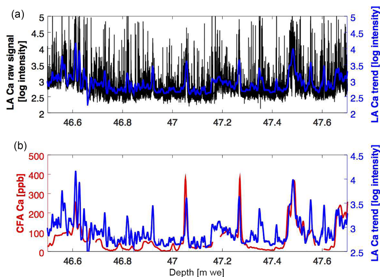
Figure 2. Ca signals obtained from the KCC ice core at around 65 % relative depth using LA-ICP-MS and CFA in direct comparison after careful alignment of the two depth scales. (a) Raw (black) and filtered LA-ICP-MS Ca signal (blue). (b) CFA Ca (red) vs. filtered LA-ICP-MS Ca signal (blue). Note (i) the additional peaks and high-frequency information revealed by LA-ICP-MS, (ii) a general agreement of CFA and low-frequency LA-ICP-MS components consistently observed over core parts measured by LA-ICP-MS. LA-ICP-MS intensity is reported as counts per second.
