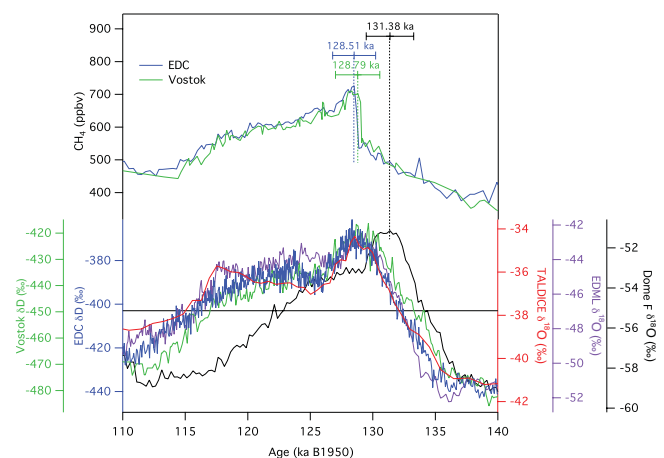
Fig. 7. Bottom: comparison of MIS 5.5 duration in several ice cores. The EDC, Vostok, EDML and TALDICE isotopic records are on AICC2012 age scales. The Dome F \delta^{18}O is on the DFO-2006 chronology (Kawamura et al., 2007). The black horizontal line corresponds to the -403 ‰ interglacial threshold on EDC. Top: methane records of Vostok and EDC. Termination II ages are defined from the timing of the sharp methane rise for EDC (blue) and Vostok (green), and the water stable isotope optima for Dome F (black).
