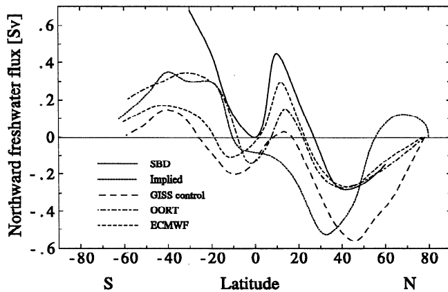
Figure 6. Implied meridional oceanic freshwater transport in the Atlantic Ocean (zonal average) derived from the zonally averaged P - E field over the drainage basin for the various data sets. The solid curve is an estimate adapted from Schmitt et al. [1992] based on oceanographic observations. The “implied” curve is the flux diagnosed from the control run of the ocean model; all lines are splines through the gridded data; positive values are northward flux in sverdrups.
