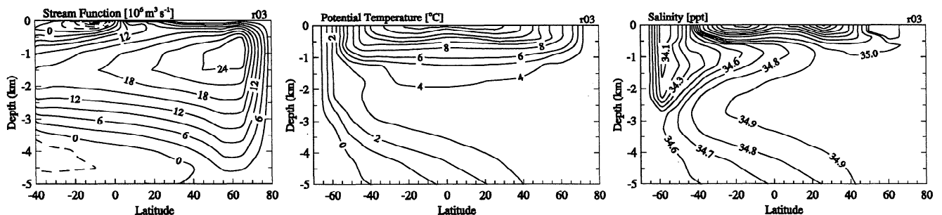
Figure 8. Meridional stream function (in sverdrups), potential temperature (in degrees Celsius), and salinity (per mil) of the model control run (restoring boundary conditions to surface salinity and temperature from Levitus [1982]) for the Atlantic basin. The clockwise meridional overturning of the thermohaline circulation is shown by the positive values of the stream function (solid lines); the high-salinity NADW ( > 34.9 ‰) has its core at about 3000 m depth; the counterclockwise cell of AABW can be seen in the deep southern part of the basin (dashed line); relatively low-salinity AAIW overlies NADW.
