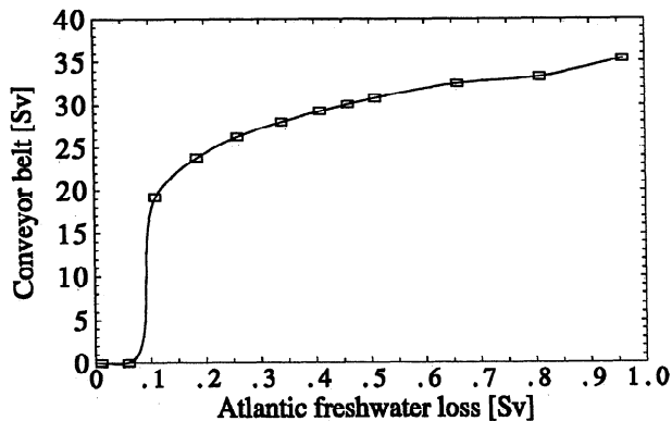
Figure 13. Strength of the thermohaline circulation as a function of the freshwater export from the Atlantic drainage basin.
