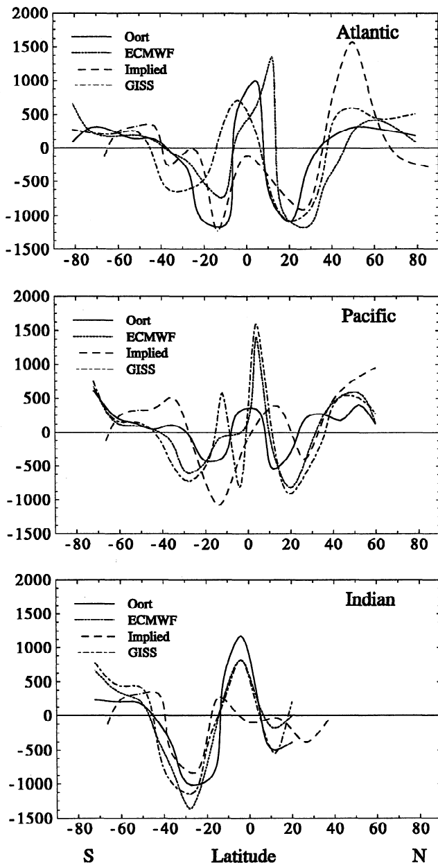
Figure 5. P - E for the Atlantic, Pacific, and Indian Oceans (from top) based on the zonally integrated convergence of atmospheric water vapor from the different data sets and the geometry of the ocean model. The “implied” curve (dashed line) is the diagnosed flux from the control run of the ocean model; all curves are splines through the gridded data; positive values are freshwater flux from the atmosphere to the ocean in mm per year.
