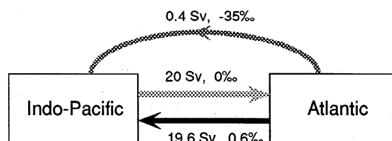
Figure 1. The importance of small changes of the atmospheric water vapor fluxes to the ocean circulation is illustrated by considering both branches of the hydrological cycle. A small atmospheric water vapor (AWV) flux with a high-salinity anomaly balances a strong oceanic transport (NADW) with a small salinity difference.
