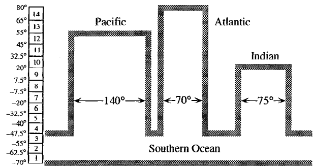
Figure 2. Geometry and resolution of the oceanic component of the climate model. Each ocean basin has area and volume that is within 5% of the observed estimates. The latitudinal resolution is shown to the left, and the vertical resolution is given in Table A1.
