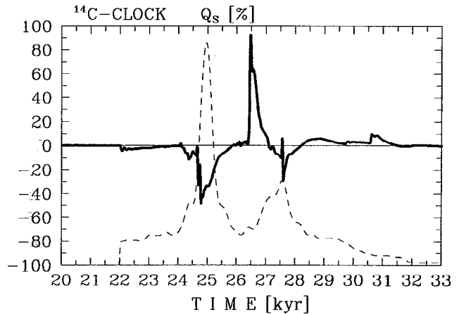
Figure 8. Evolution of the slowdown of the radiocarbon clock, Q_s , for experiment C2. The rise of ^{14}\text{C}^{\text{atm}} causes an “acceleration” of the clock, while reinitiation of the ventilation produces a slowdown. The meltwater discharge into the North Atlantic is shown by the dashed line on a scale of 0–0.5 Sv.
