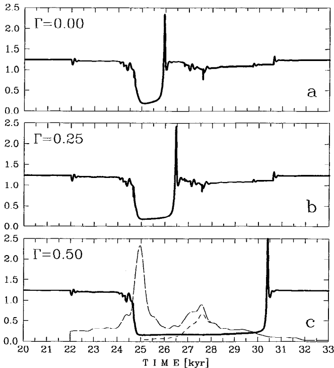
Figure 4. Evolution of the Atlantic meridional heat flux across 32.5^\circ\text{N} in petawatts ( 1 \text{ PW} = 10^{15} \text{ W} ). Shown are cases in which the runoff into the North Atlantic at high latitudes is reduced to (a) 0.00 (experiment C1), (b) 0.25 (experiment C2) and (c) 0.50 (experiment C3) of present-day values as the heat flux is reduced to zero. The meltwater discharges into the North Atlantic and Southern Ocean are indicated by the long- and short-dashed lines, respectively, on a scale of 0–0.5 Sv. The second, weaker meltwater peak appears to be due to a reduction of the ice volume of Antarctica [Peltier, 1994]. This is taken into account by linearly increasing the fraction of Southern Ocean meltwater input from 0% to 50% at the expense of the North Atlantic input over the 3000 years following the first meltwater peak.
