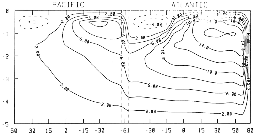
Fig. 14. Quasi-steady thermohaline circulation in the Pacific-Atlantic basin system. The Pacific (Atlantic) basin extends from 50° N to 61° S (80° N to 61° S) and is 5000 m deep; contours of the meridional stream function are in 10^6 \text{ m}^3/\text{s} . The main region of sinking is in the North Atlantic from where the deep water spreads into the Pacific, where it upwells. The results are obtained using a two-basin version of the zonally averaged ocean model of Wright and Stocker (1991).
