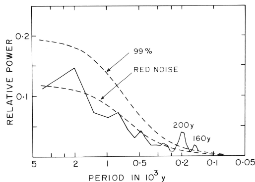
Fig. 6. Spectrum of the La Jolla tree ring \delta^{14}\text{C} record (solid line) with the spectrum of the first-order autoregressive process and the associated 99% confidence limit. [From Neftel et al. , 1981.]
