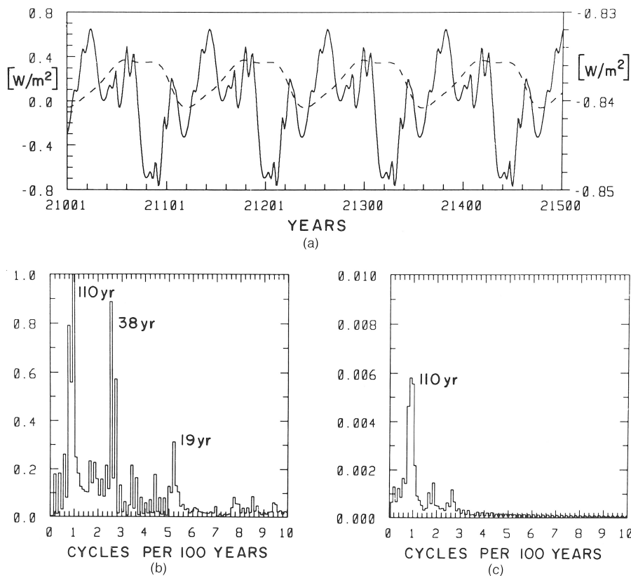
Fig. 15. (a) Time series of the average ocean-to-atmosphere heat flux in W/m^2 of the Atlantic ( 55^\circ S to 80^\circ N , solid, left ordinate) and Pacific ( 55^\circ S to 50^\circ N , dashed, right ordinate). Under steady surface forcing natural variability occurs in the form of a self-sustained oscillation. (b) Normalized power spectrum of the time series in (a) for the Atlantic. (c) Power spectrum of the time series in (a) for the Pacific. The total variance in the Pacific is about 100 times smaller than in the Atlantic.
