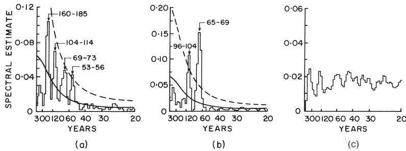
Fig. 3. Power spectra of the oxygen-isotope records covering the past 800 yr from Camp Century (a), Crête (b) and Devon (c). The Greenland cores (a) and (b) show peaks of the century time scale that are close to or exceeding the 95% confidence limit (dashed line) of the corresponding first-order autoregressive process (solid line). The record of Devon Island (northern Canada) shows no cycles and resembles white noise. [From Stuiver, 1980.]
