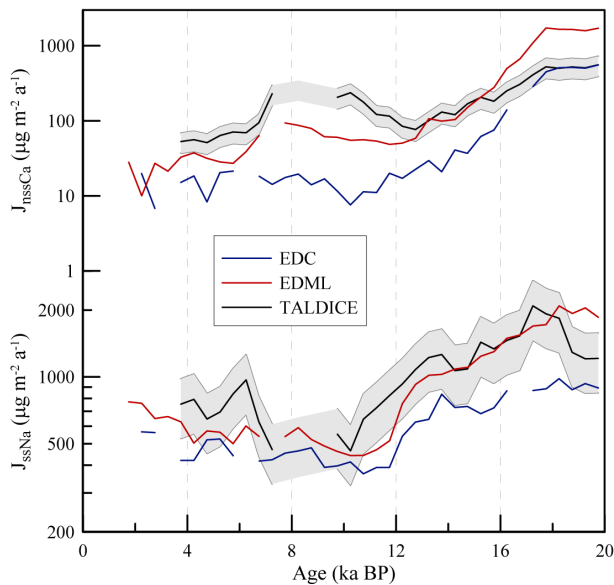
Fig. 4. \text{NssCa}^{2+} ( J_{\text{nssCa}} ) and \text{ssNa}^+ ( J_{\text{ssNa}} ) fluxes for the Holocene and T1. The grey shaded bands indicate the range covered by the estimated 30% error as mentioned in Sect. 2.3. In TALDICE, they show opposite trends during the deglaciation and early–mid-Holocene (i.e. 13–6 ka BP).
