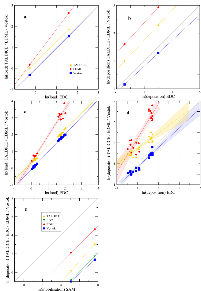
Fig. 7. (a) Dust column load of 1 yr tuned model runs at ice core grid points (Albani et al., 2012b). Double-logarithmic plots at EDML (red diamonds), Vostok (blue squares), and TALDICE (yellow triangles) vs. EDC. (b) Double-logarithmic plots of modelled dust deposition for all drill sites. The results are from the same model run as in (a). (c) Results of two 10 yr simulations showing inter-annual variability (10 points for each climate period) of the dust column load. Double-logarithmic scatter plots at EDML (red diamonds), Vostok (blue squares), and TALDICE (yellow triangles) vs. EDC, with the linear regressions including significance intervals (95 %) indicated in respective colours. See Table 2 for slopes, standard deviations, and r^2 values of the regressions shown in this figure. (d) Double-logarithmic plots of two 10 yr simulations for all drill sites showing inter-annual variability of the dust deposition. The results are from the same model run as in (c). Linear regressions including significance intervals (95 %) are indicated in respective colours. (e) Double logarithmic scatter plot of the source mobilisation vs. deposition showing the relation of dust deposited at the four ice core sites originating from a unique source (South America, SAM) based on the 1 yr tuned case of Albani et al. (2012b). Green triangles represent EDC.
