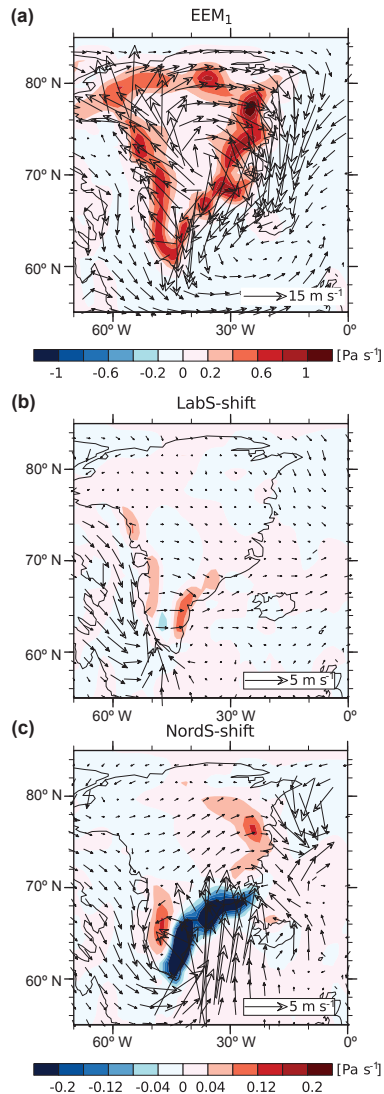
Figure 9. Winter (DJF) mean vertical (shaded) and horizontal (vectors) wind velocities at lowest terrain-following model level for (a) \text{EEM}_1 , (b) LabS-shift response, and (c) NordS-shift response. Positive (negative) vertical wind velocities denote downward (upward) motion.
