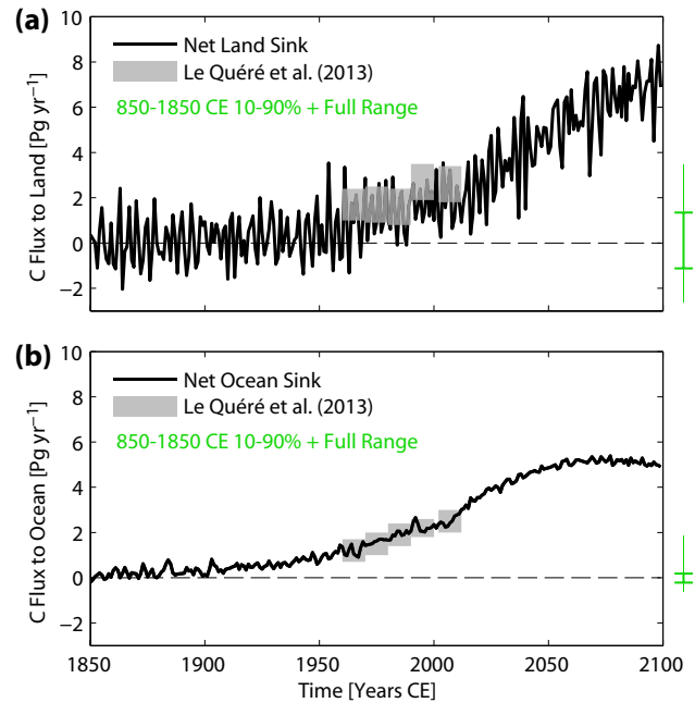
Figure 4. Annual mean net carbon flux from the atmosphere to (a) land and (b) ocean. Green bars given the full and 10–90% range from the preindustrial part of the simulation. Observational estimates are from Le Quéré et al. (2013).
