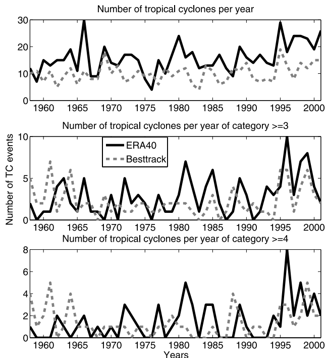
Figure 4. (top) Number of all TCs, (middle) hurricanes of category three and more and (bottom) hurricanes of category four and five per season after the fitting in the Atlantic basin in ERA-40 (black line) and best track (gray dashed).
