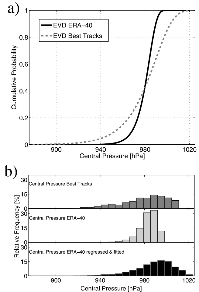
Figure 3. (a) EVDs of all best track central pressures (gray dashed) and all ERA-40 regressed central pressures (black line). (b) Central pressures of all tracks of best track (gray), ERA-40 (light gray) and fitted and regressed ERA-40 (black).
