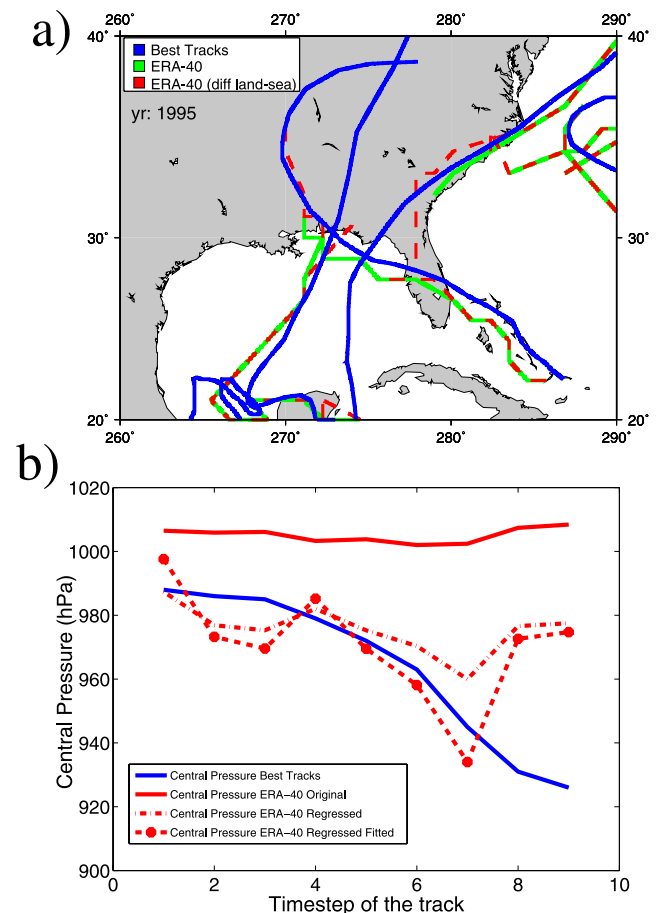
Figure 2. Case studies: (a) Tracks over land of the hurricane season (June–November) 1995 with the best tracks of NHC (blue), the adapted uniform tracking technique in ERA-40 (green) and the adapted tracking technique with different land-sea tracking (red dashed). (b) Central pressures of one exemplary cyclone from 08/31/1977 to 09/02/1977 from best track (blue), calculated with the tracking tool and ERA-40 (red), ERA-40 regressed (red dashed) and ERA-40 regressed and fitted (red dotted and dashed).
