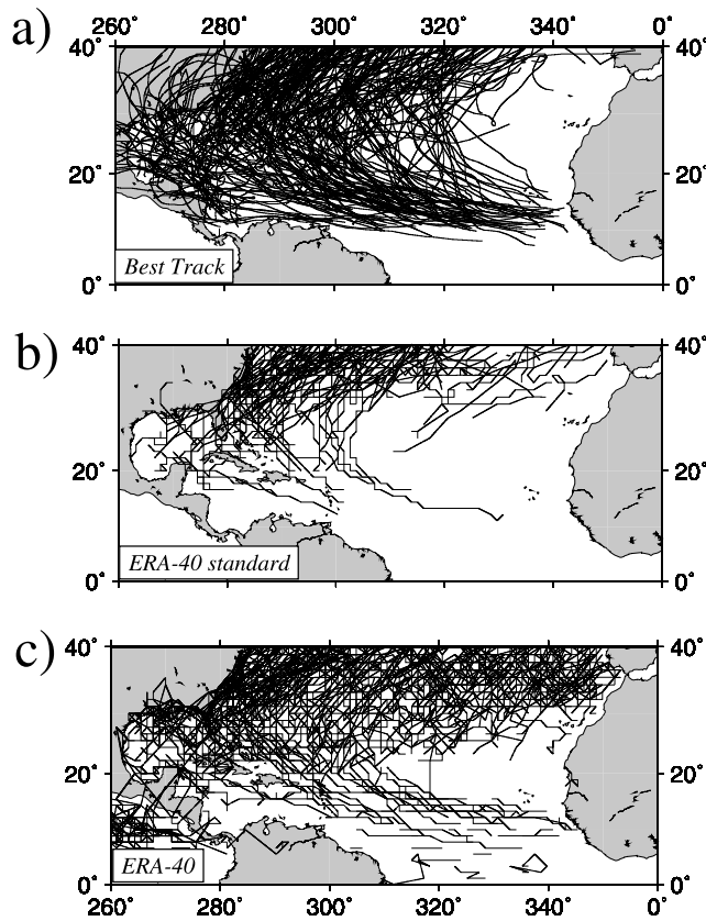
Figure 1. Tracks of all hurricane seasons (June–November) from 1958 through 2001 with (a) the best tracks of NHC, (b) the standard tracking technique of midlatitudes, and (c) the adapted tracking technique with different land-sea tracking.
