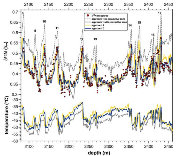
Fig. 7. Top panel: \delta^{15}\text{N} measurements (red dots) and firm model calculations versus ice depth. Bottom panel: Surface temperature evolution used as model input. The different approaches are described in the text. (For interpretation of the references to colour in this figure legend, the reader is referred to the web version of this article.)
