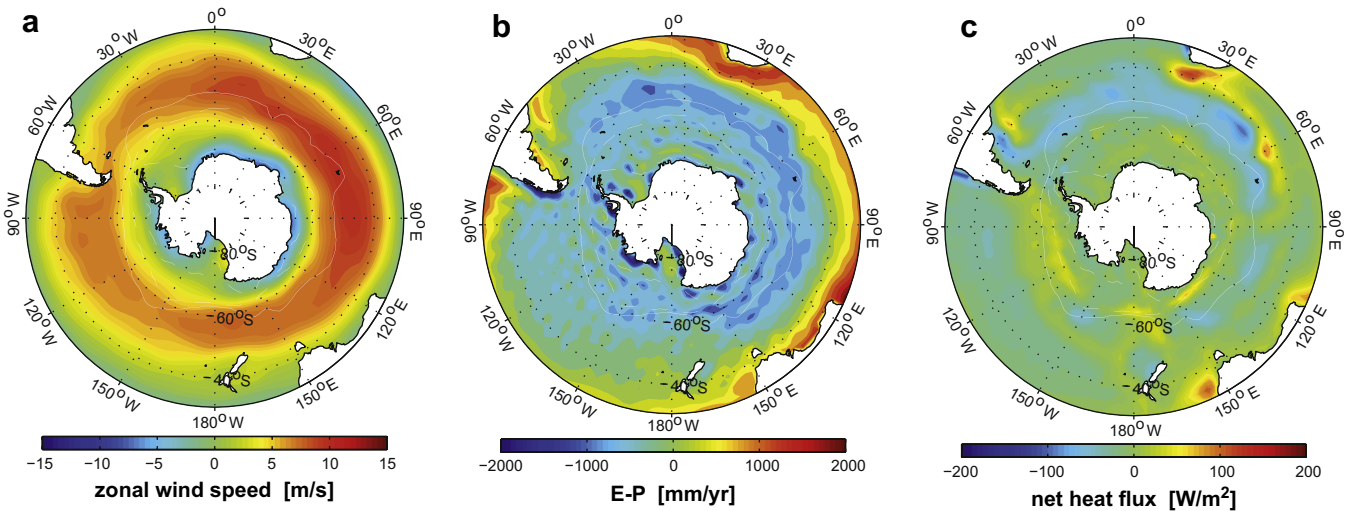
Fig. 6. a) Zonal wind speed, b) evaporation minus precipitation (E-P) with evaporation estimated from the latent heat flux, c) surface net heat flux calculated from the sum of net shortwave and net longwave radiation, sensible heat flux and latent heat flux (net downward heat fluxes taken as negative) in the Southern Ocean region, derived from NCEP/NCAR reanalysis data (Kalnay et al., 1996). Note that the reanalysis data are model dependent. Furthermore, b) represents only the vertical freshwater exchange with the atmosphere and no salt/freshwater fluxes due to sea ice formation and melting are included. Accordingly, b) and c) are given only to provide an overall picture of the zonal and meridional structure but cannot be directly compared to the buoyancy fluxes in Fig. 7. Dashed white lines represent the current summer and winter sea ice edge, while the solid white line indicates the average position of the modern PF. In the glacial, the position of the winter sea ice edge is close to the position of the modern PF.
