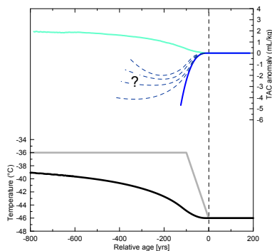
Figure 11. Modeled behavior of TAC for an idealized DO event with a 10^\circ\text{C} linear surface warming during 100 years after the onset of the event. At the bottom, in grey, the assumed surface temperature and in black the temperature at bubble close-off depth. At the top, in turquoise, the TAC model output for steady-state firnification conditions (Eq. 11). Blue: the transient firnification model (Schwander et al., 1997) TAC output for a constant bubble close-off time. Dashed lines indicate the range of measured TAC anomalies.
