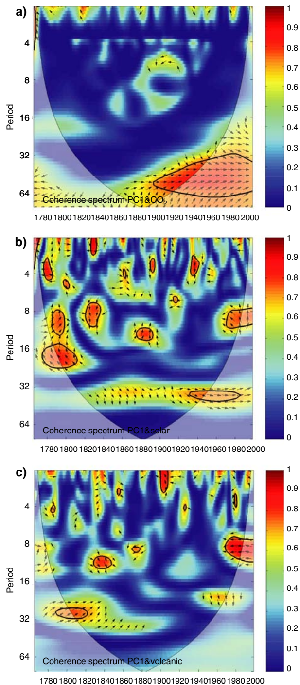
Fig. 7 a–c The squared wavelet coherence between the PC1 and a the CO 2 forcing (Etheridge et al. 1996), b the solar forcing (Lean et al. 1995; Crowley 2000), and c the volcanic forcing (Crowley 2000). The thick black contour is the 5% significance level against red noise. The cone influence where edge effects might be relevant is indicated as lighter shadings. The coloured shading varies from zero to one, where one means perfect correlation in the time-frequency space. Arrows indicate the phase shift (the convention is: pointing right = in-phase; pointing left = anti-phase; pointing straight up = the PC1 leads the forcing by 90 degrees). More details about the method are found in Grinsted et al. (2004)
