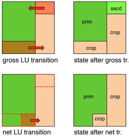
Fig. 1. Schematic illustration of simulating gross versus net land use change. Under a scheme for gross land use change (upper row), land is claimed and abandoned for/from use as cropland in parallel within one gridcell. Under a scheme for net land use change (lower row), only the difference of claimed minus abandoned undergoes a transition to use as cropland. In the latter scheme, a smaller gridcell area fraction is affected by land use change.
