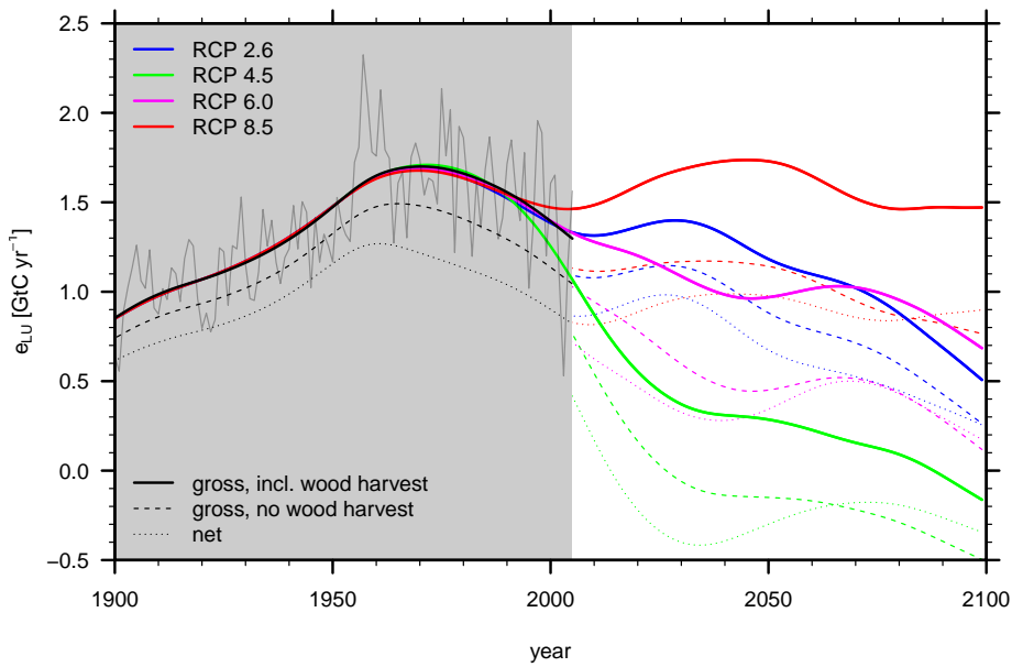
Fig. 5. Annual LUC fluxes for 1900-2100 and the different RCPs. Thick black and colored curves are splined time series of annual data, which is shown by the thin solid curve for the past. Dashed and dotted lines represent annual LUC fluxes, diagnosed from a simulation without wood harvesting and from a simulation where only net land use change is simulated, respectively.
