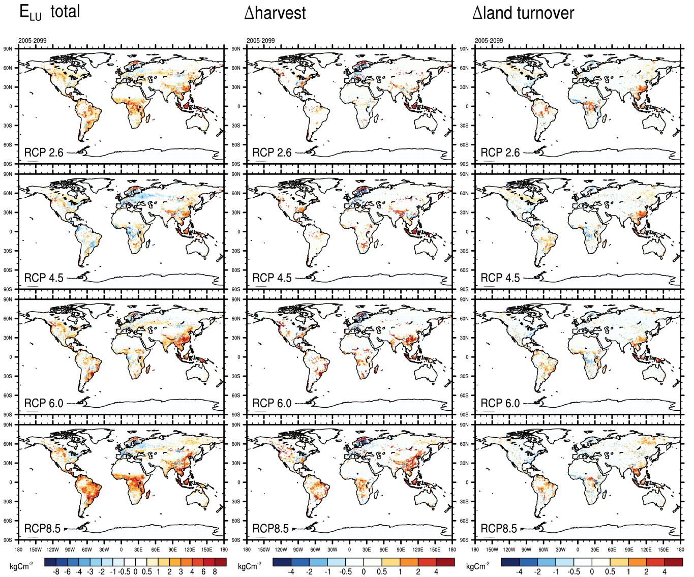
Fig. 6. Spatial distribution of cumulative future (RCPs) LUC emissions and its components. Left: Total (gross, incl. wood harvest) cumulative LUC emissions in \text{kgC}/\text{m}^2 middle: Cumulative emissions due to wood harvest. Right: Effect of land turnover (including the introduction of secondary land) as the difference between the run with gross LU transitions and a run with net LU transitions; both runs do not consider wood harvest. Note the different color scales in the panels.
