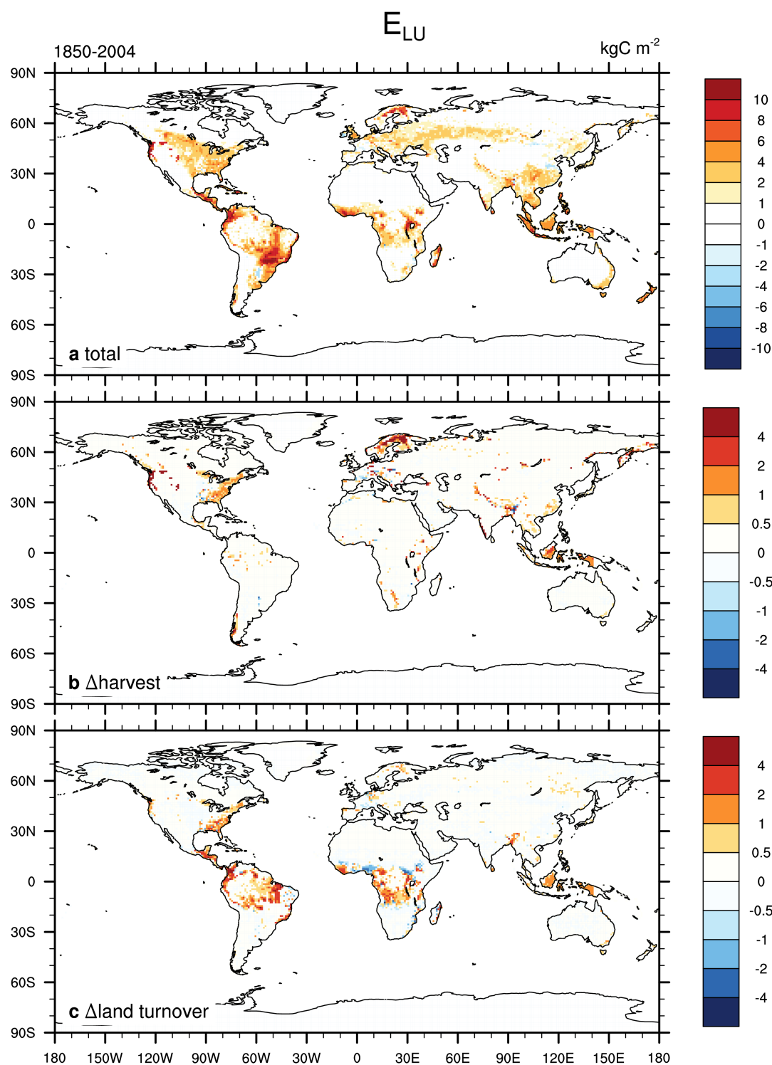
Fig. 4. Spatial distribution of cumulative historical (1850-2004) LUC emissions and its components. a : Total (gross, incl. wood harvest) cumulative LUC emissions in kgC/m^2 . b : Cumulative emissions due to wood harvest. c : Effect of land turnover (including the introduction of secondary land) as the difference between the run with gross LU transitions and a run with net LU transitions; both runs do not consider wood harvest. Note the different color scales in the upper and the lower two panels.
