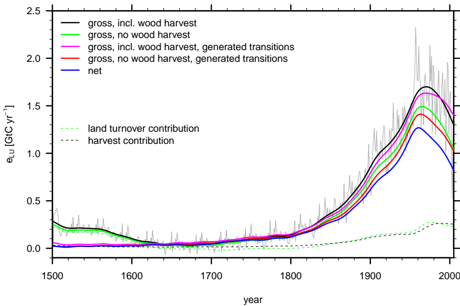
Fig. 2. Historical annual LUC fluxes. Splined annual fluxes (thick color lines) and year-by-year data for “gross, incl. wood harvest” (thin grey line) are shown. The dashed lines (“land turnover contribution” and “wood harvest contribution”) are the differences between the respective curves (“land turnover contribution” = “gross, no wood harvest” – “net”; “wood harvest contribution” = “gross, incl. wood harvest” – “gross, no wood harvest”)
