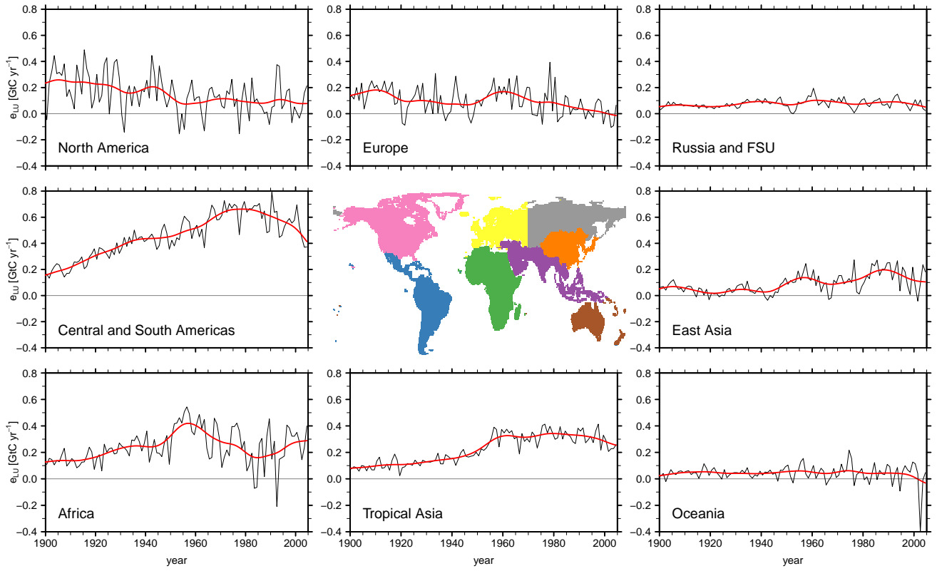
Fig. 3. Annual LUC fluxes by region (black curves) and their splined time series (red curve). The regions are illustrated by the map in the middle and correspond to the delineation used in IPCC AR5 (Ciais et al., 2013), except that “Eurasia” is separated into Europe (everything west of 60°E), and Russia and the Former Soviet Union (FSU) (everything east of 60°E).
