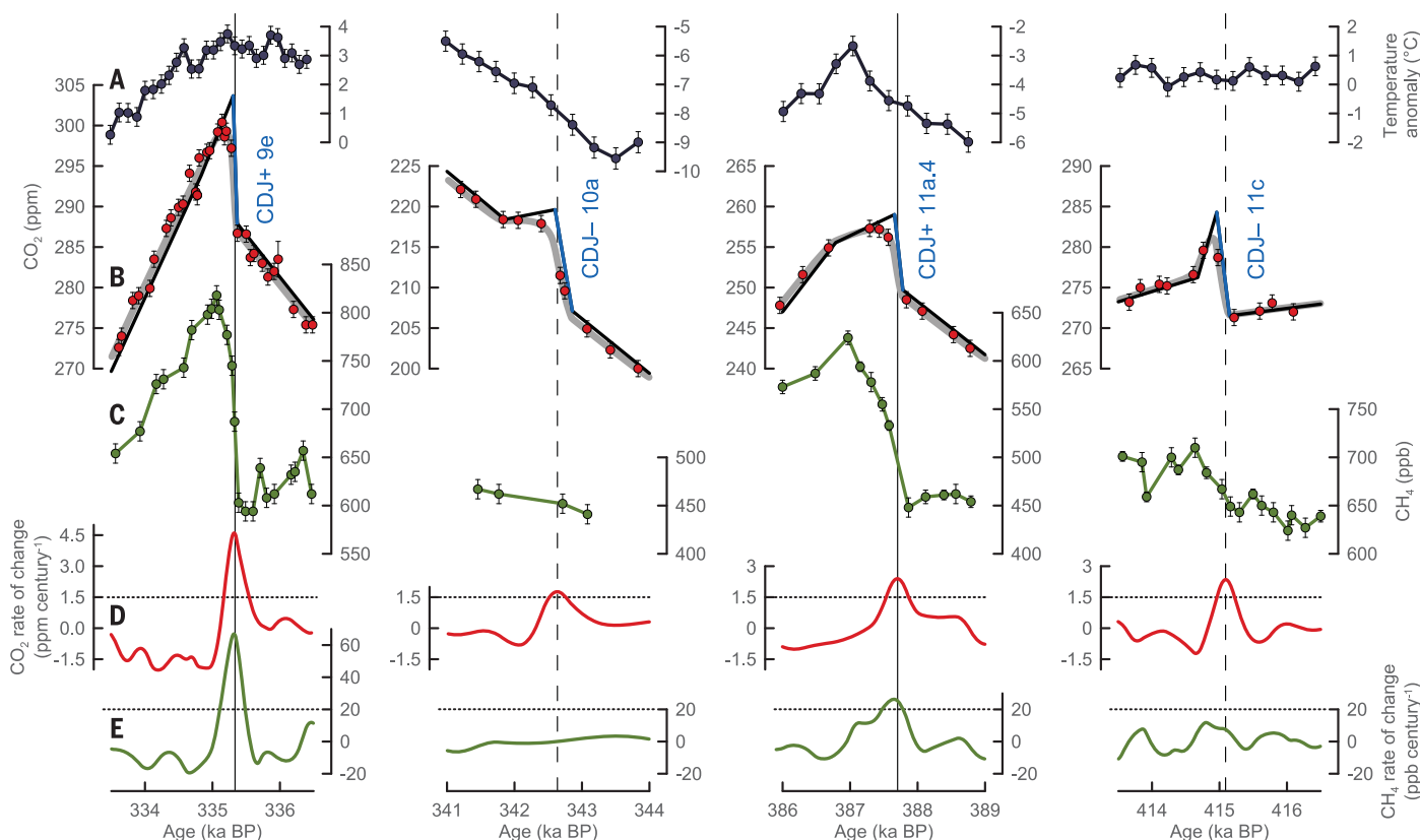
Fig. 3. Detailed view of the two varieties of CDJ. (A to E) Identical to Fig. 1. The black linear segments in (B) indicate first-order approximations of the atmospheric CO 2 evolution. The blue segment highlights the actual CDJ event. These approximations for the atmospheric trajectories are optimized so that the
