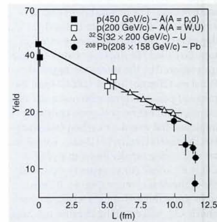
The yield of J/ψ as a function of the length L of the path of the preresonant state through nuclear matter. Drell-Yan events, i.e. , promptly produced muon pairs in the mass continuum, are used as a reference since their yield exhibits the normal expected behaviour. The Pb data are plotted in 5 centrality bins.
