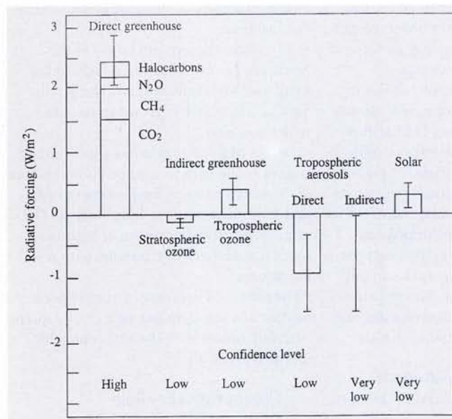
Fig. 1. Estimates of the globally averaged radiative forcing owing to changes in the concentrations of greenhouse gases and aerosols from pre-industrial times to the present day and changes in solar variability since 1850. The radiative forcing of a radiative agent is defined as the additional downward flux into the lower atmosphere mediated by an instantaneous increase of the agent's concentration. The height of the bars indicates a mid-range estimate of the forcing while the bars themselves show the possible range of values. An indication of the relative confidence in the estimates is given below each bar. The negative values for aerosols should not necessarily be regarded as an offset against the greenhouse gas forcing since aerosols are distributed unevenly over the globe. From [1].
