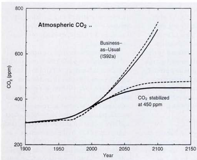
Fig. 6. Atmospheric CO 2 concentration as calculated with the "Bern" carbon cycle model for the central "Business-as-Usual" scenario (IS92a) of the Intergovernmental Panel on Climate Change (IPCC). The scenario depends on assumptions about population growth, economic growth, and various other factors. According to this scenario, carbon emissions increase from a present level of about 7 GtC/yr to about 20 GtC/yr by the end of the next century. Concentration profiles to limit atmospheric CO 2 at 450 ppm have also been developed by IPCC to illustrate emissions and climate change consequences (Fig. 7, 8). In addition to CO 2 , other radiative forcing agents such as methane, nitrous oxide, halocarbons and aerosols are important. The dashed lines give the total radiative forcing of all relevant anthropogenic greenhouse gases and aerosols. For comparison, the total forcing has been expressed in units of CO 2 (equivalent). The relationship between CO 2 concentration and radiative forcing - forcing (W/m 2 ) = 6.3 ln (CO 2 /280 ppm) - allows one to convert the radiative forcing of other greenhouse gases and aerosols into units of CO 2 (equivalent). The radiative forcing of non-CO 2 greenhouse gases happens to be roughly offset by the negative forcing due to aerosols. Uncertainties surrounding future emissions of aerosol precursor gases and related radiative forcing are large.
