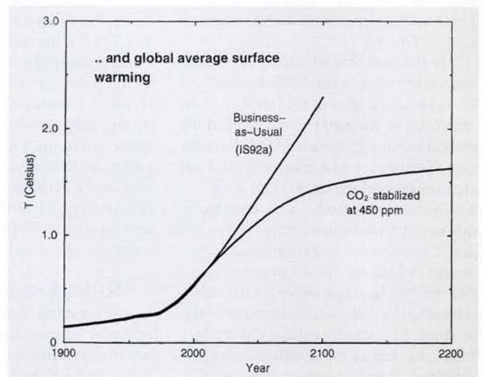
Fig. 7. Global average surface warming as calculated by the "Bern" model for the IS92a scenario and for the profile (Fig. 6, dashed lines) for stabilizing CO 2 at 450 ppm. The model is used to calculate the oceanic heat uptake. The temperature sensitivity is prescribed to be 2.5°C for a doubling of atmospheric CO 2 . This is the central value of sensitivities estimated by atmosphere general circulation models. The temperature continues to increase even after CO 2 stabilization as it takes many centuries to warm up the ocean.
