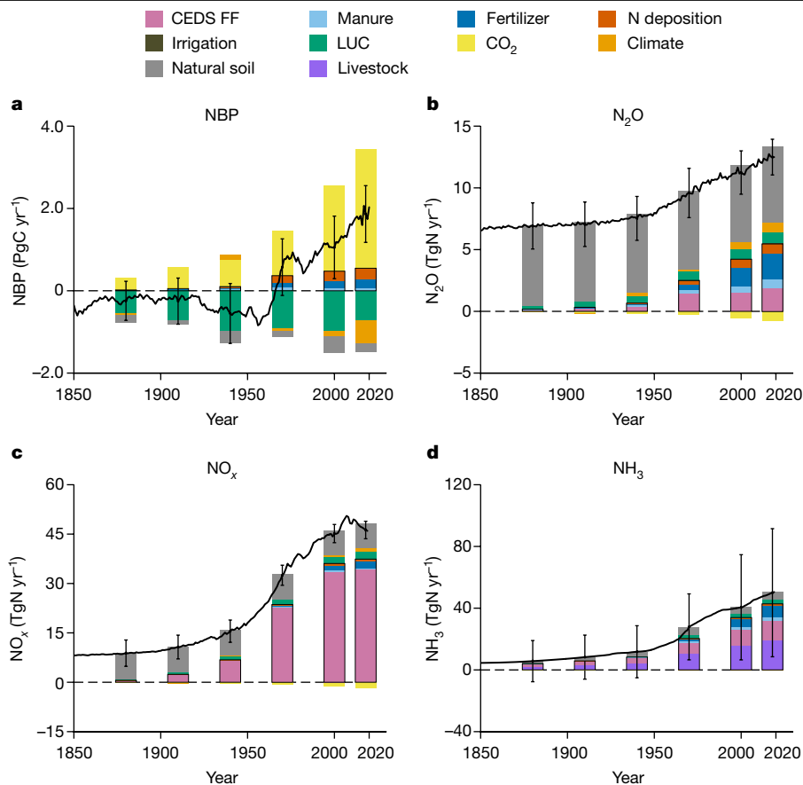
Fig. 2 | Historical N r emissions and terrestrial carbon fluxes based on CEDS inventory and NMIP2 ensemble mean. a–d. The terrestrial NBP (a), N 2 O (b), NO x (c) and NH 3 (d) emissions, respectively. All of the fossil fuel sources in CEDS are indicated by the pale violet bars, whereas other colours indicate factor contributions based on the NMIP2 ensemble mean. The soil NH 3 emissions have been scaled by the CEDS agricultural emissions (Methods). The fire emission of
