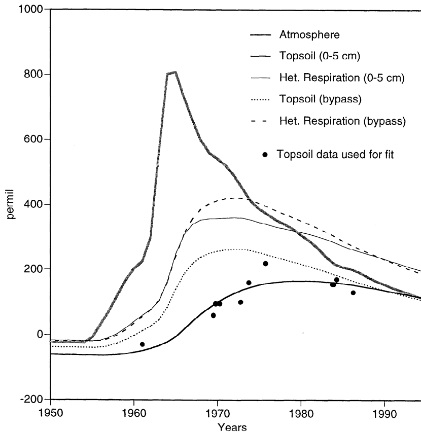
Figure 3. Effect of litter mineralization and humification on simulated ^{14}\text{C} in soil and heterotrophically respired \text{CO}_2 at Meathop Wood for a soil depth of 5 cm. Atmospheric ^{14}\text{C} data for the Northern Hemisphere are from Enting et al. [1994]. Note the higher levels of simulated ^{14}\text{C} if plant litter is bypassed ("bypass" simulation) compared to the data of Harkness et al. [1986] for the early 1970s and the convergence of the two simulations in the late 1980s. All ^{14}\text{C} data are expressed in \text{‰}\Delta^{14}\text{C} .
