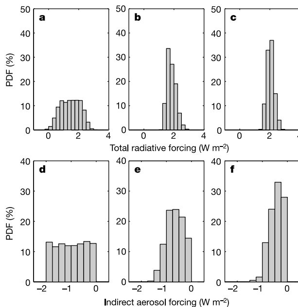
Figure 2 Constraints on the radiative forcing from the observed atmospheric and oceanic warming. Probability density functions (PDF) for the total (anthropogenic and natural) radiative forcing ( a–c ) and the indirect aerosol forcing ( d–f ) in the year 2000 are based on 25,000 Monte Carlo simulations. The initially assumed PDFs are given in a and d . The requirement that the model matches the temperature observations strongly narrows the PDFs ( b and e ). If in addition the climate sensitivity is restricted to the range adopted by the IPCC (1.5–4.5 K), the PDFs in c and f are obtained.
